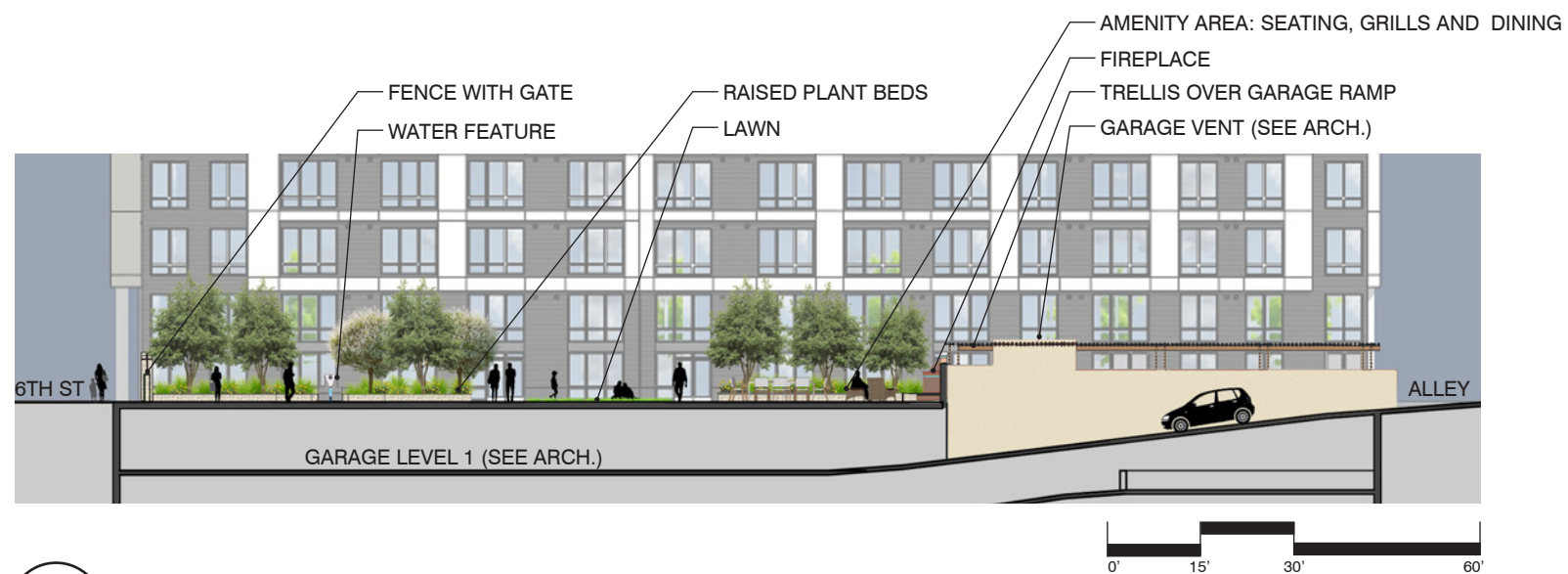
1 SECTION - NORTH COURTYARD L-14
