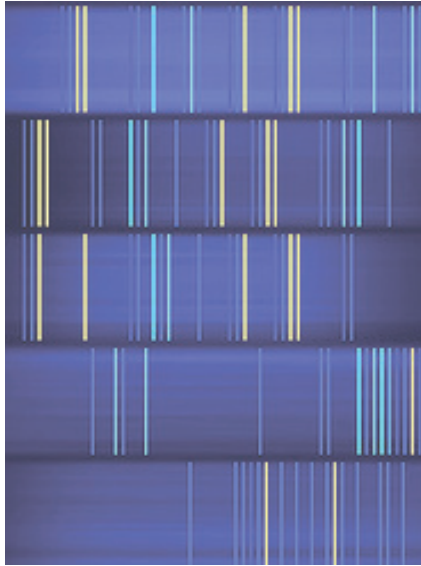
Genome sequencing
