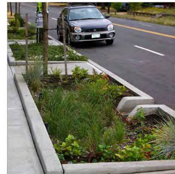
STORMWATER DIRECTED INTO BIORETENTION PLANTER
