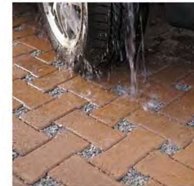
UNIT PAVERS OVER PERMEABLE BASE COURSE
