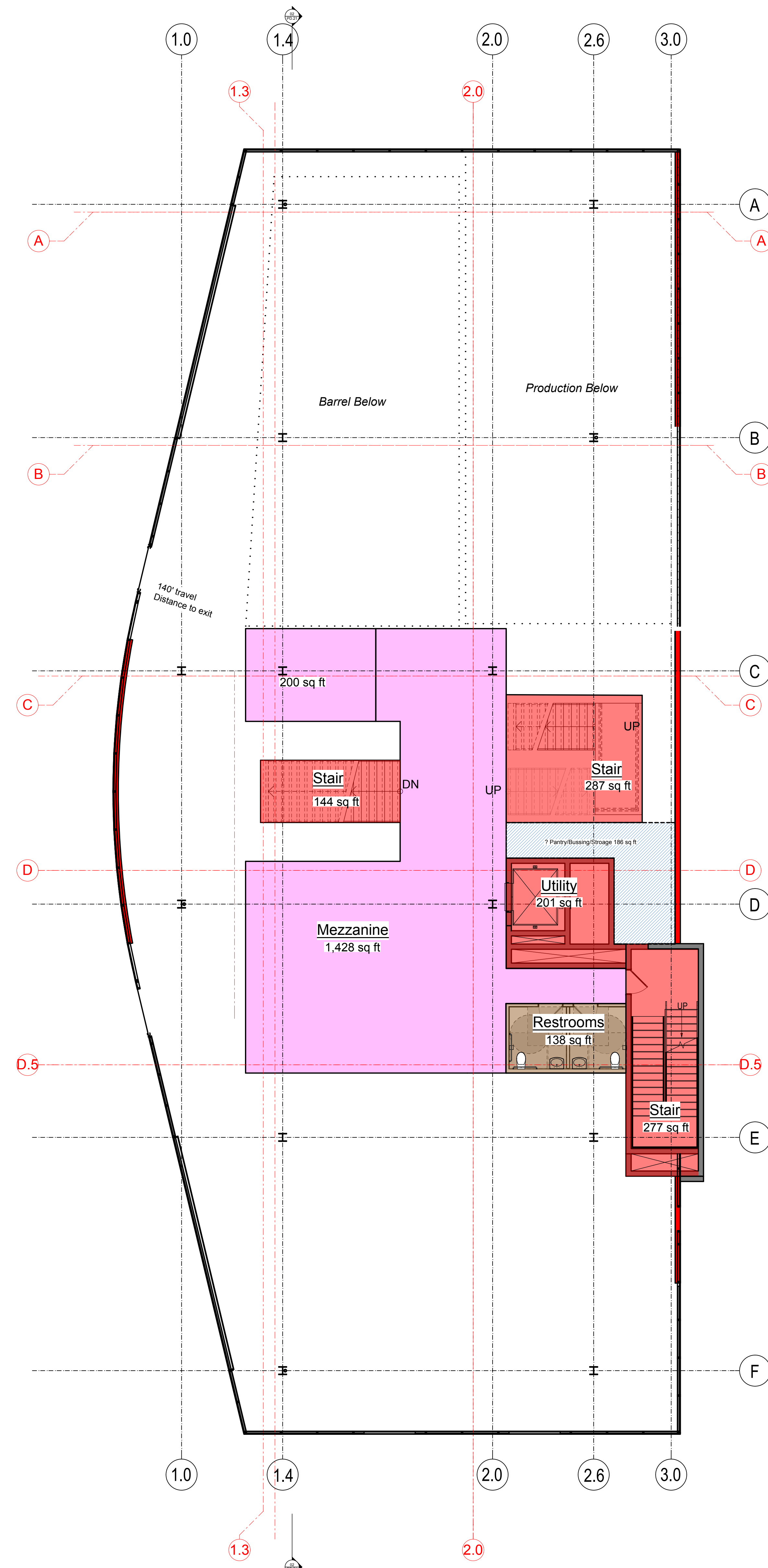
02 Program Layout Mezzanine (District Winery) Scale: 1/8" = 1'-0"
