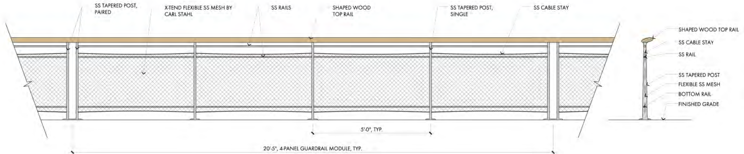
GUARDRAIL ELEVATION
