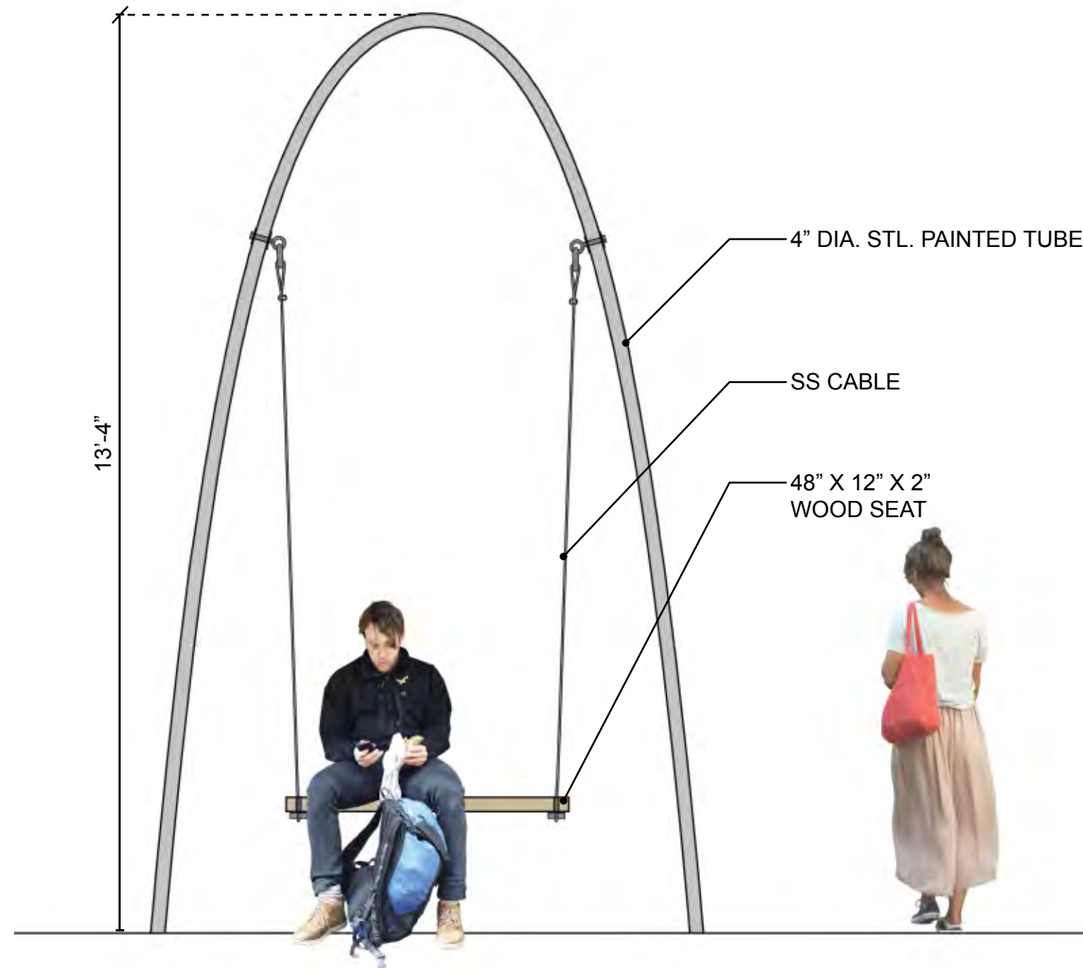
SWING ELEVATION
