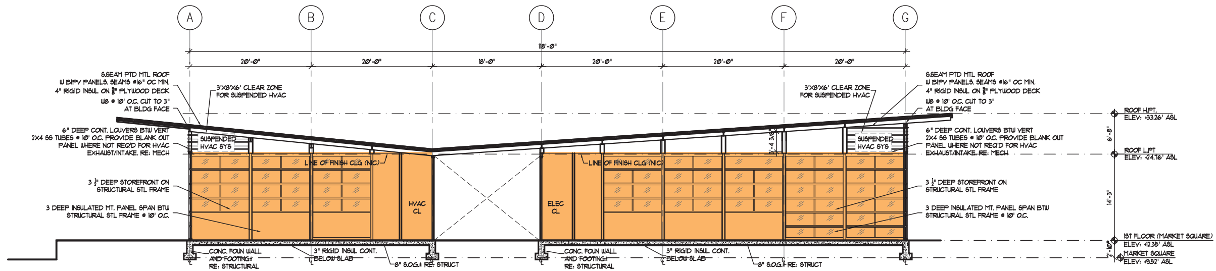
SECTION
