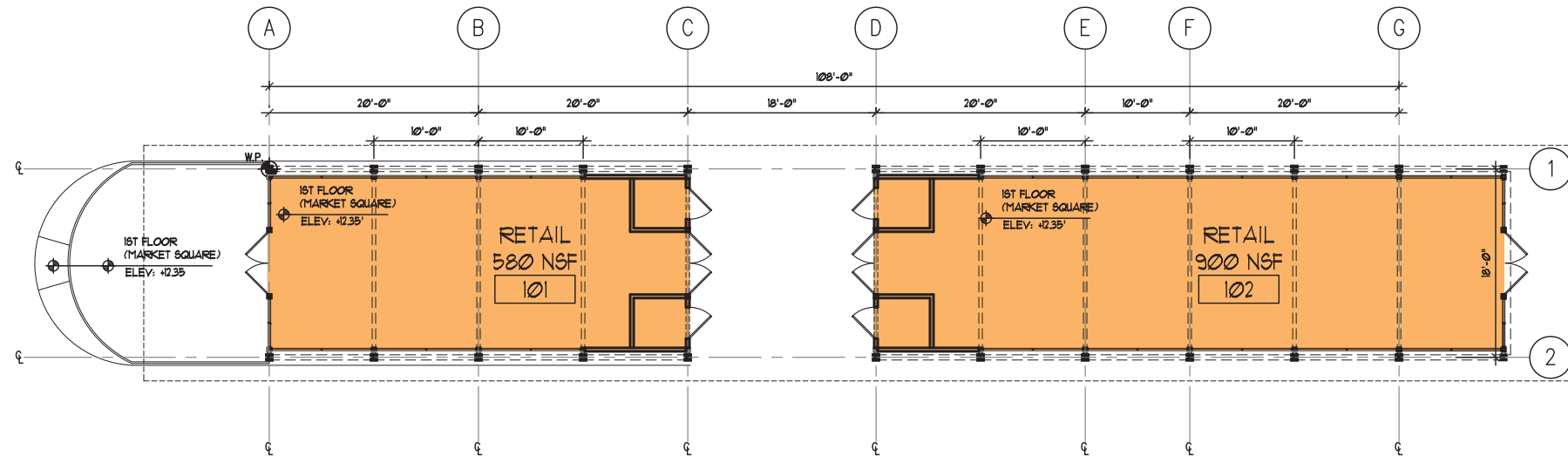
GROUND LEVEL PLAN
