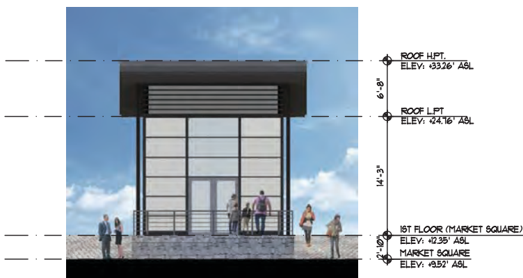
SOUTH ELEVATION
