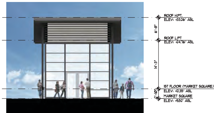
NORTH ELEVATION
