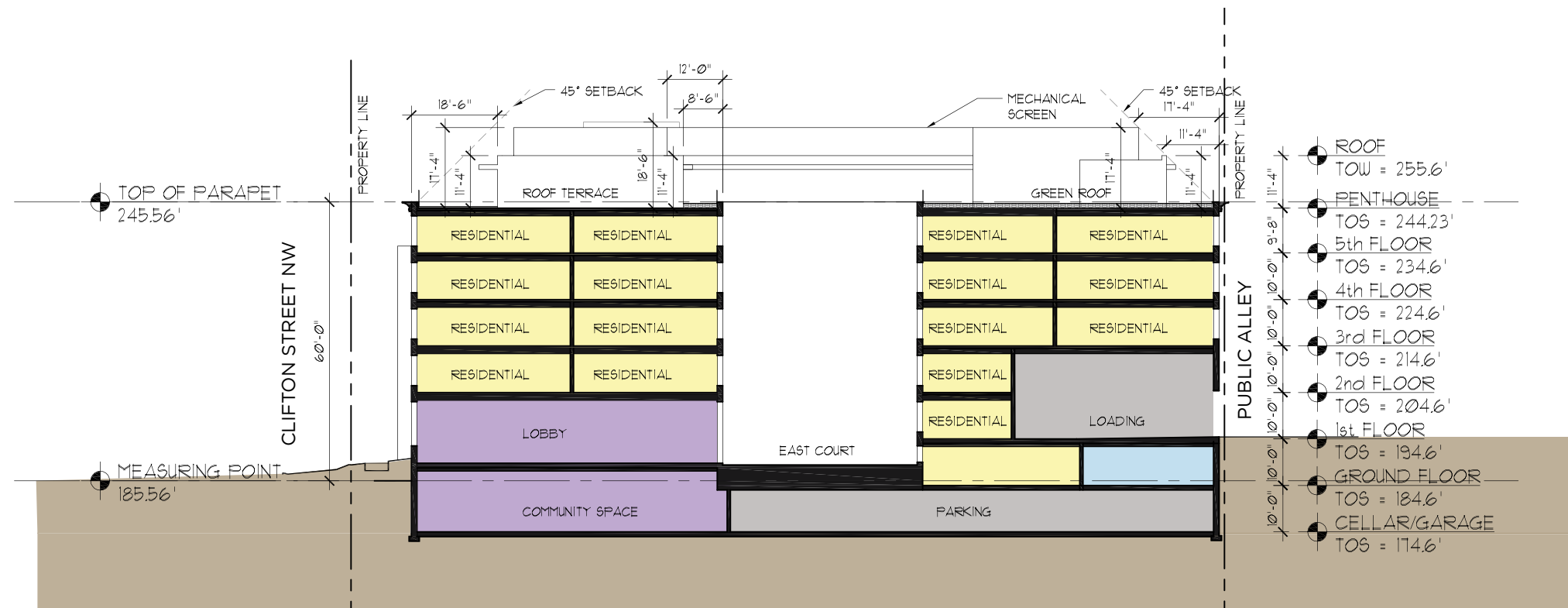
SECTION C-C 1" = 32'-0"
