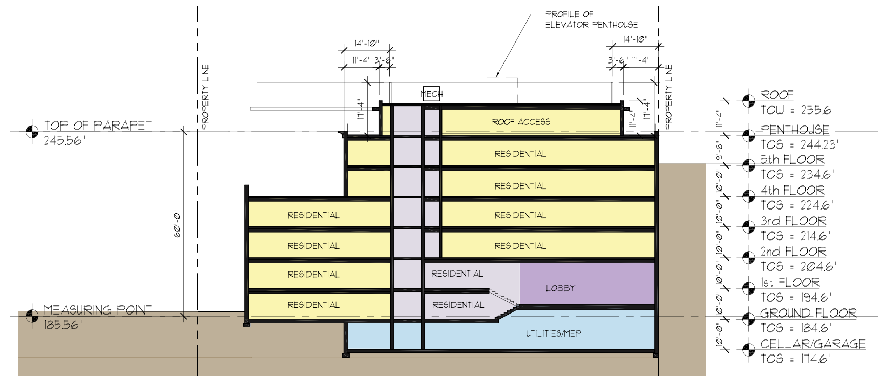
SECTION D-D 1" = 32'-0"
