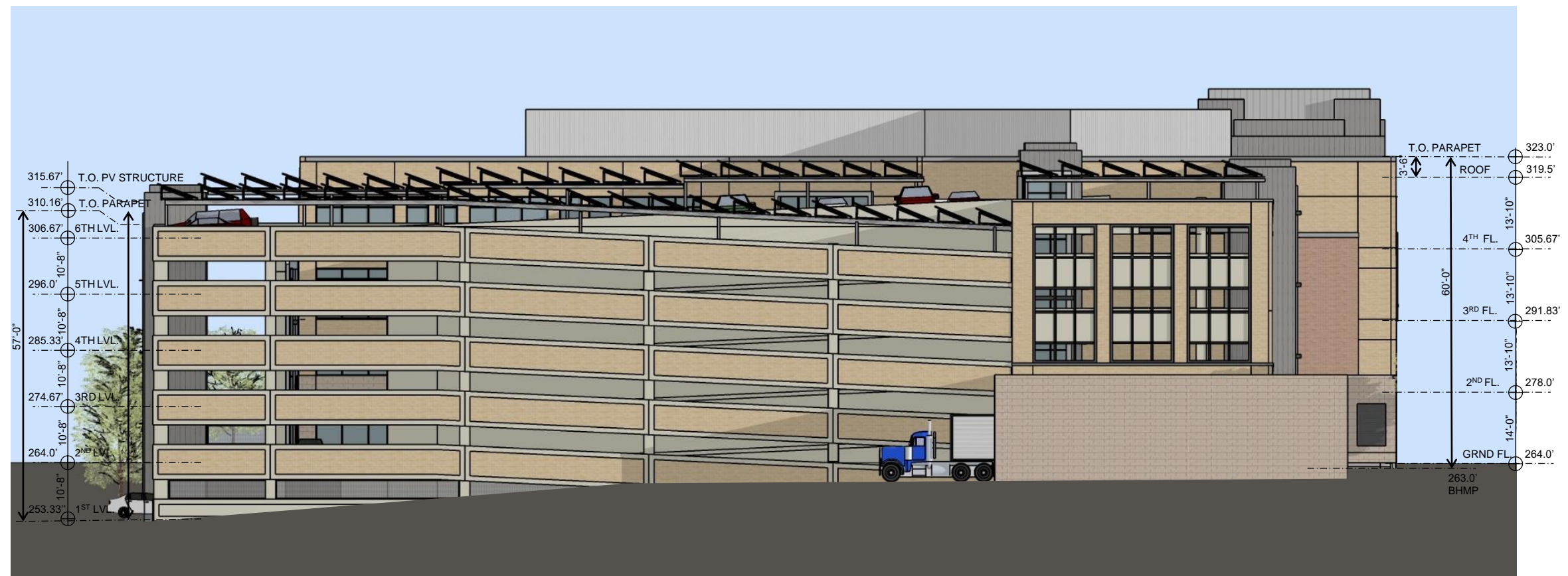
South Elevation
