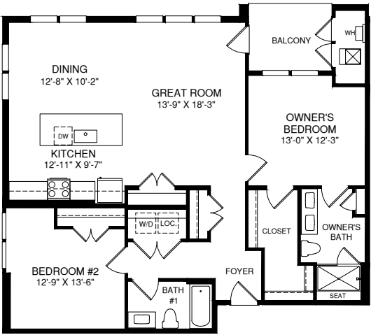
LAYOUT 2- RUBY
