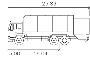
Garbage Truck
