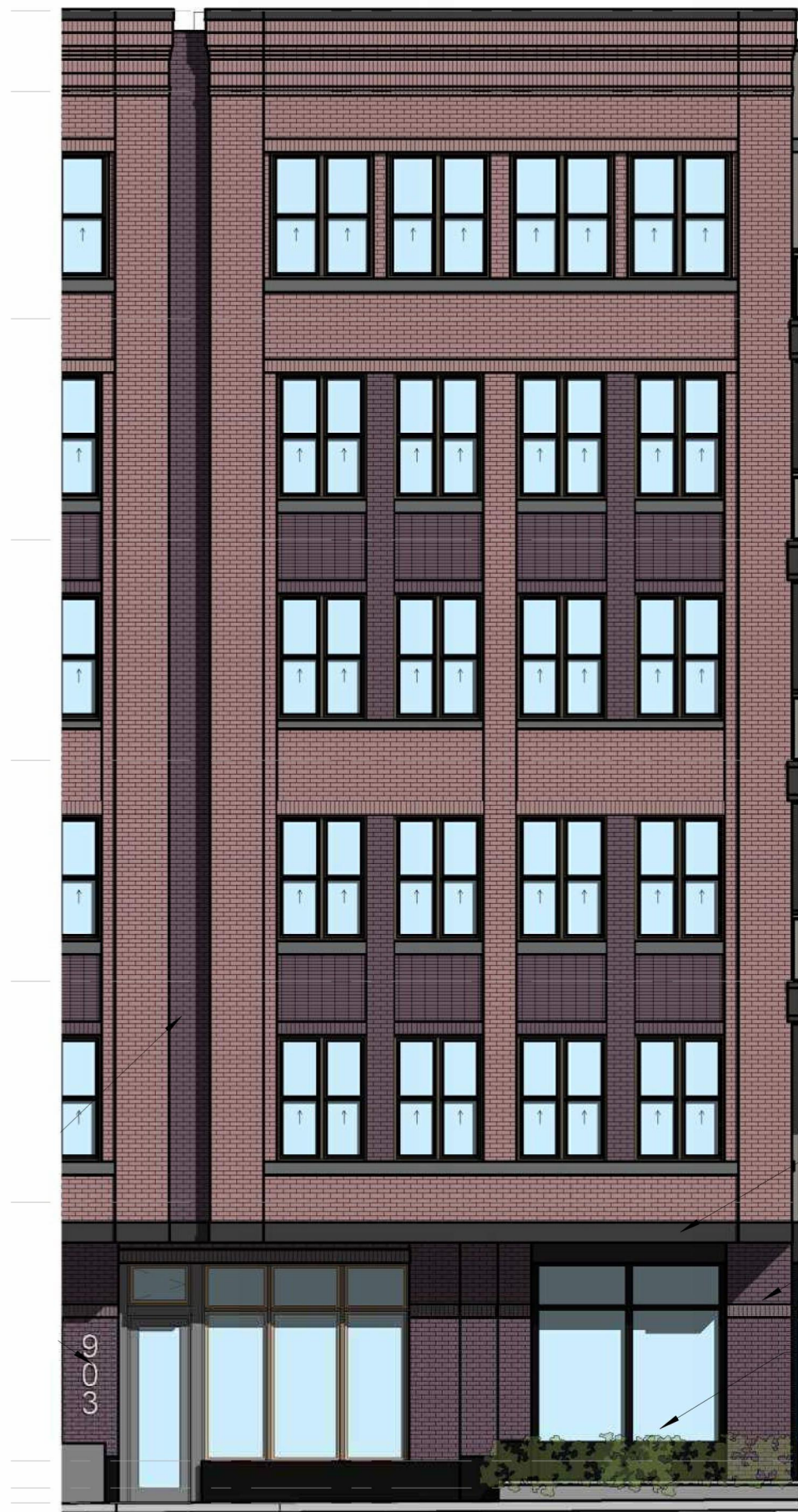
② North Elevation - Typical Bay of Live/Work Units - BEFORE 1/8" = 1'-0"
