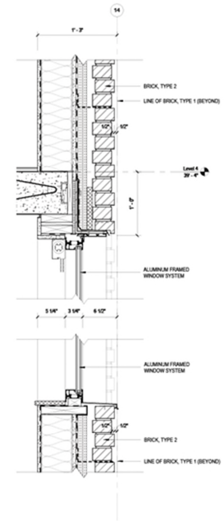
DETAIL SECTION
