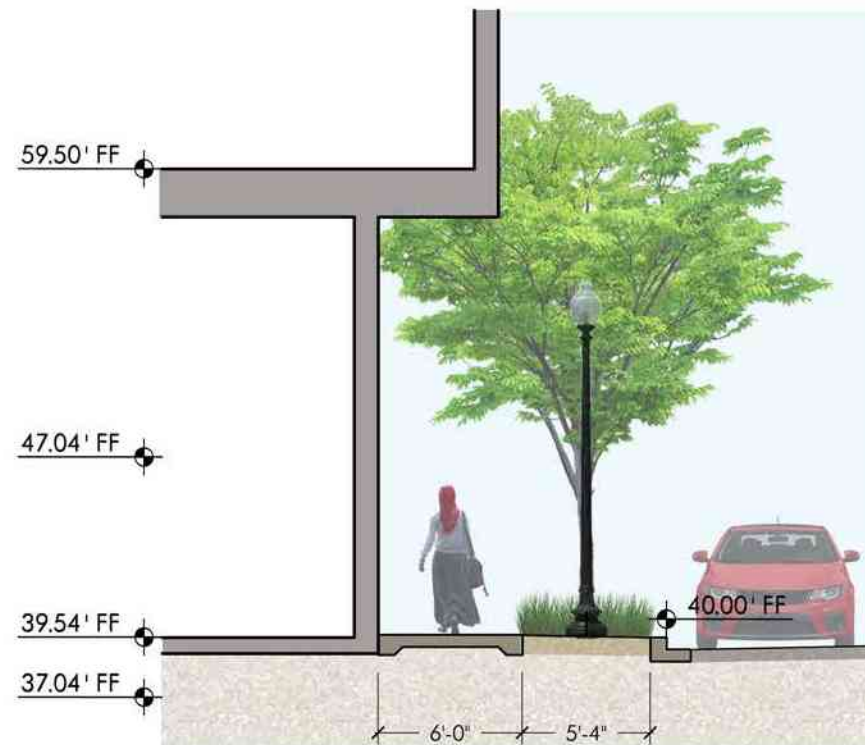
SECTION 4 - L STREET NW SCALE: 1/8"=1'-0"
