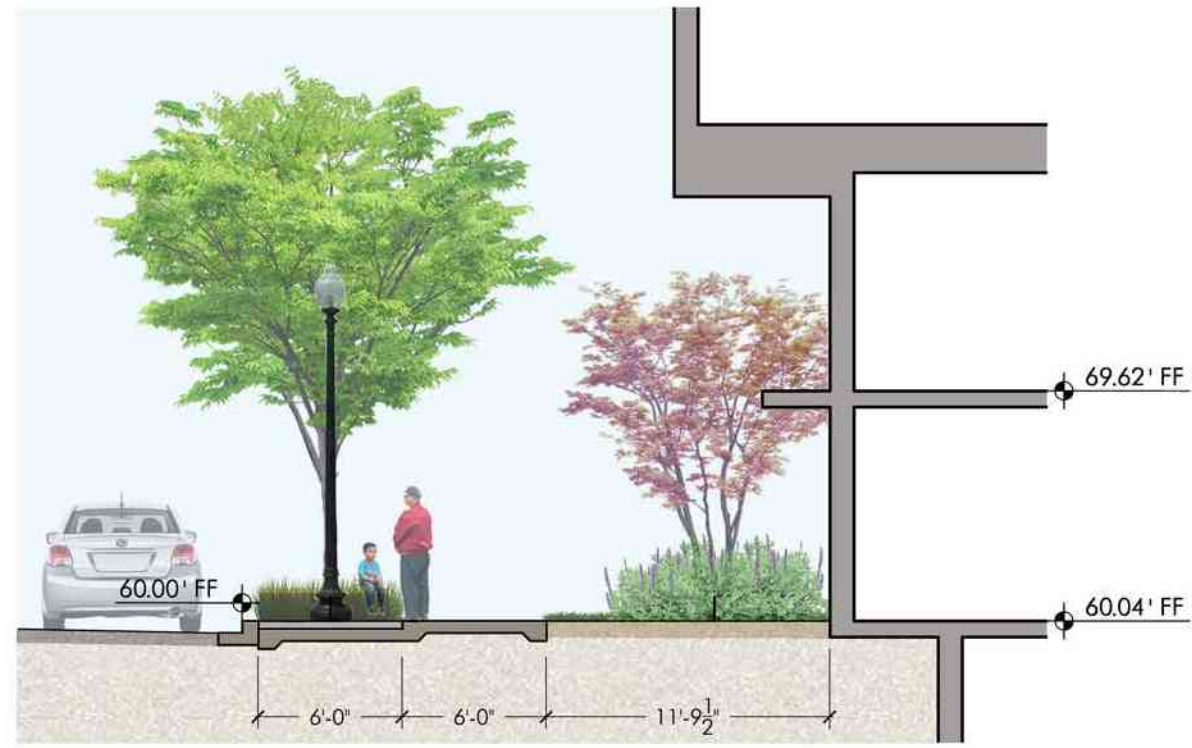
SECTION 2 - PIERCE STREET NW SCALE: 1/8"=1'-0"
