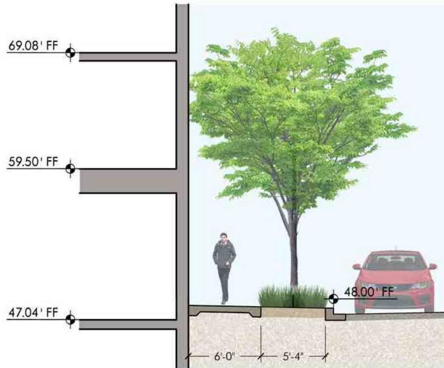
SECTION 3 - 1ST PLACE STREET NW SCALE: 1/8"=1'-0"
