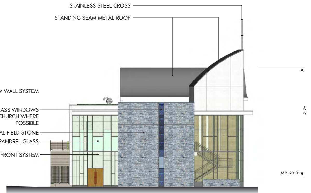
CHURCH ELEVATION ALONG 7TH STREET
