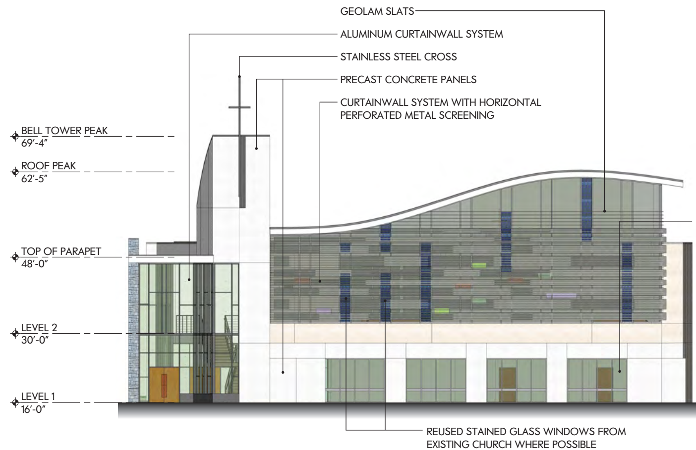
CHURCH ELEVATION ALONG MAINE AVE
