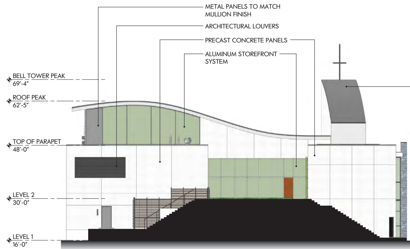
CHURCH ELEVATION AT COURTYARD
