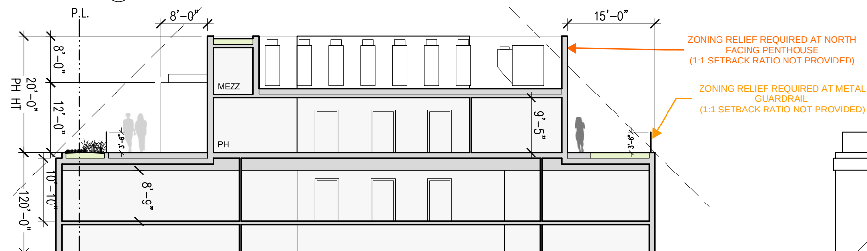
Ⓑ - SOUTH / NORTH ROOFTOP SECTION
