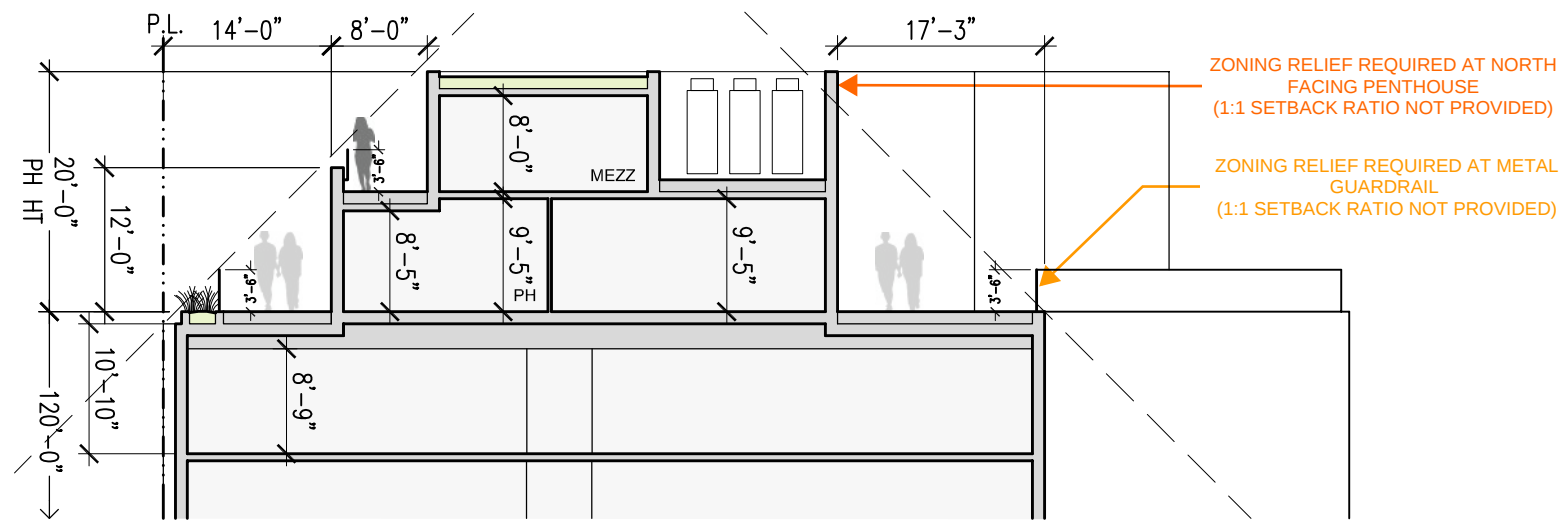
Ⓐ - SOUTH / NORTH ROOFTOP SECTION
