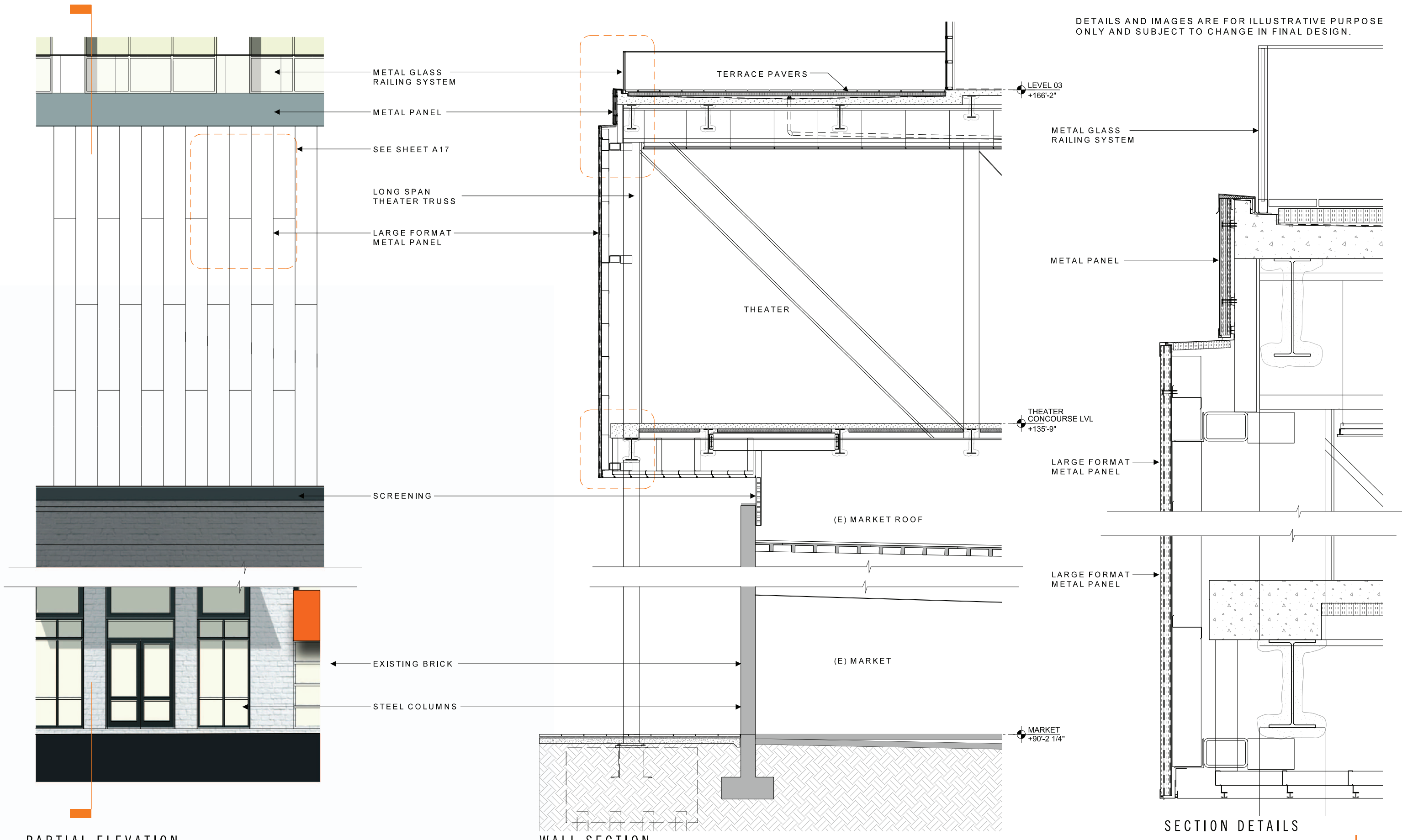
PARTIAL ELEVATION
