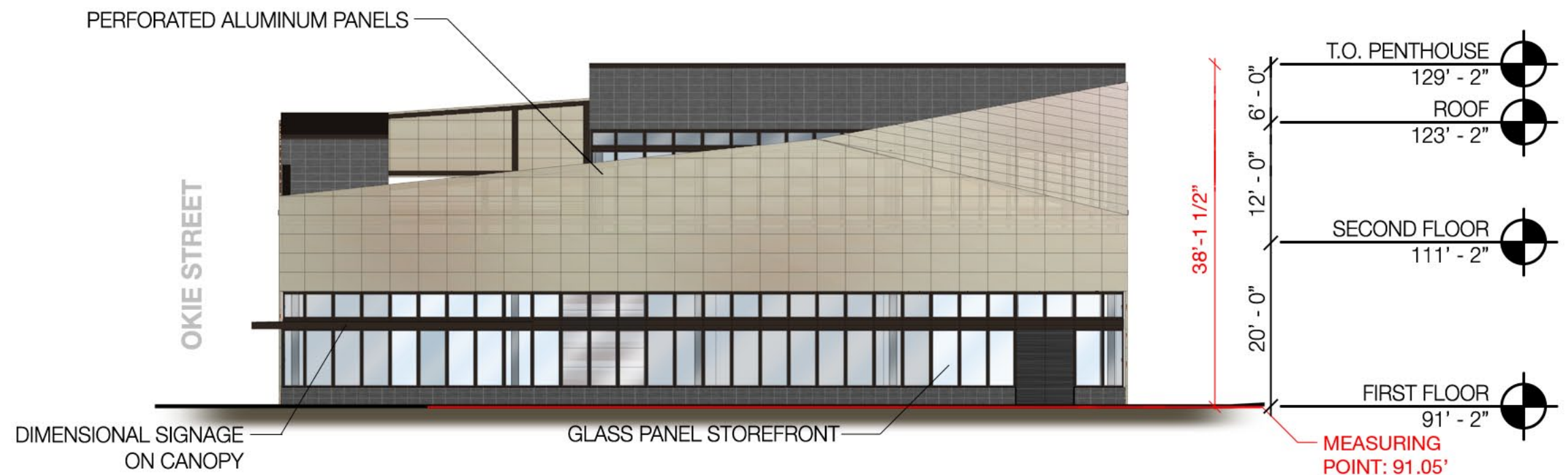
SOUTH ELEVATION
