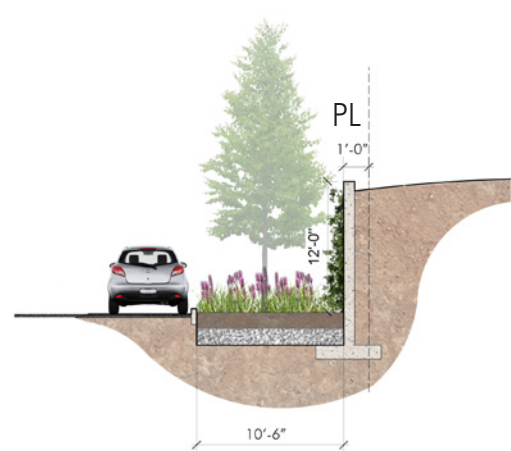
SECTION F 12' WALL
