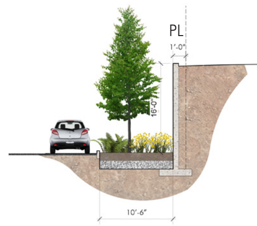
SECTION E 16' WALL
