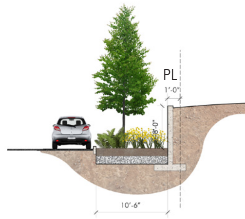
SECTION G 8' WALL
