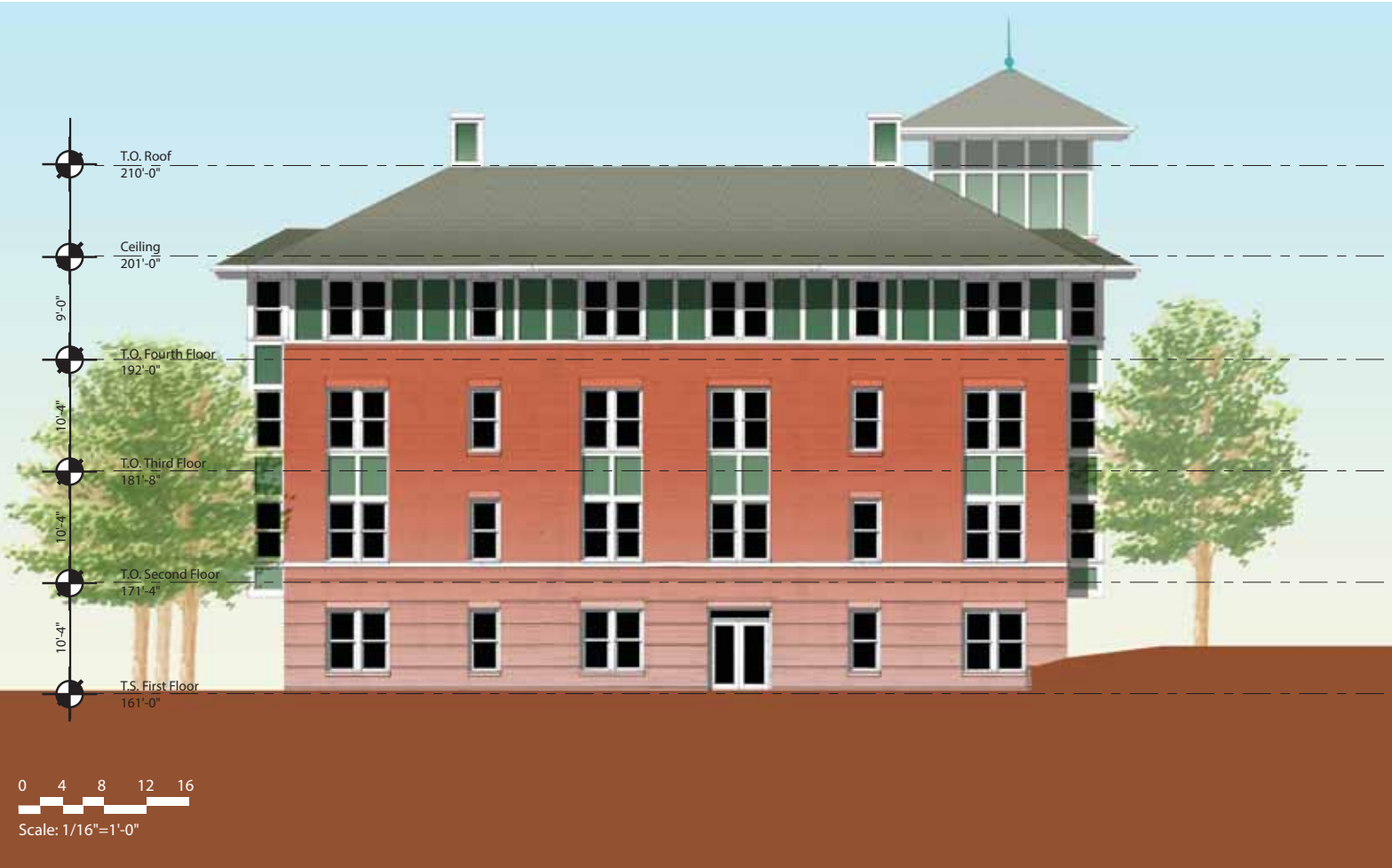
Building A East Elevation
