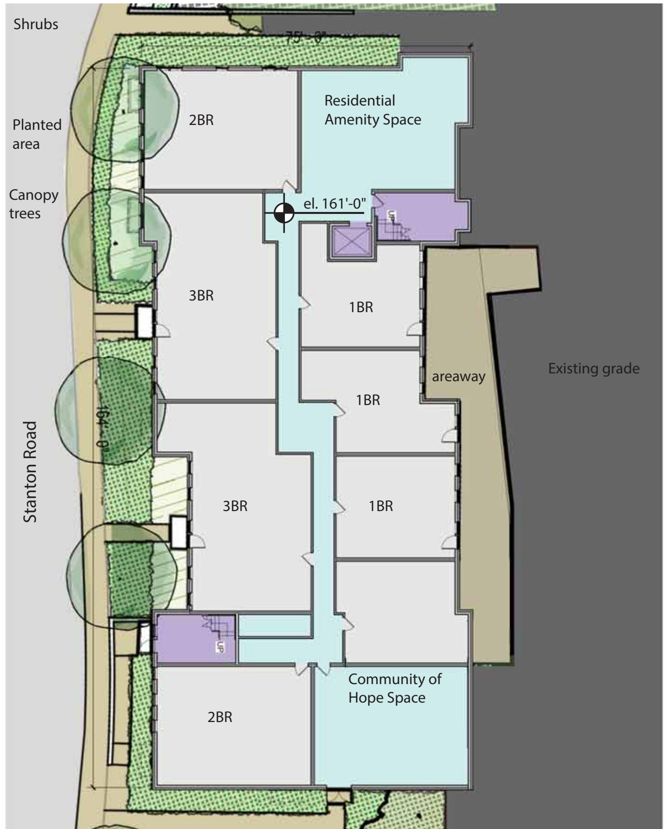
Building A First Floor Plan
