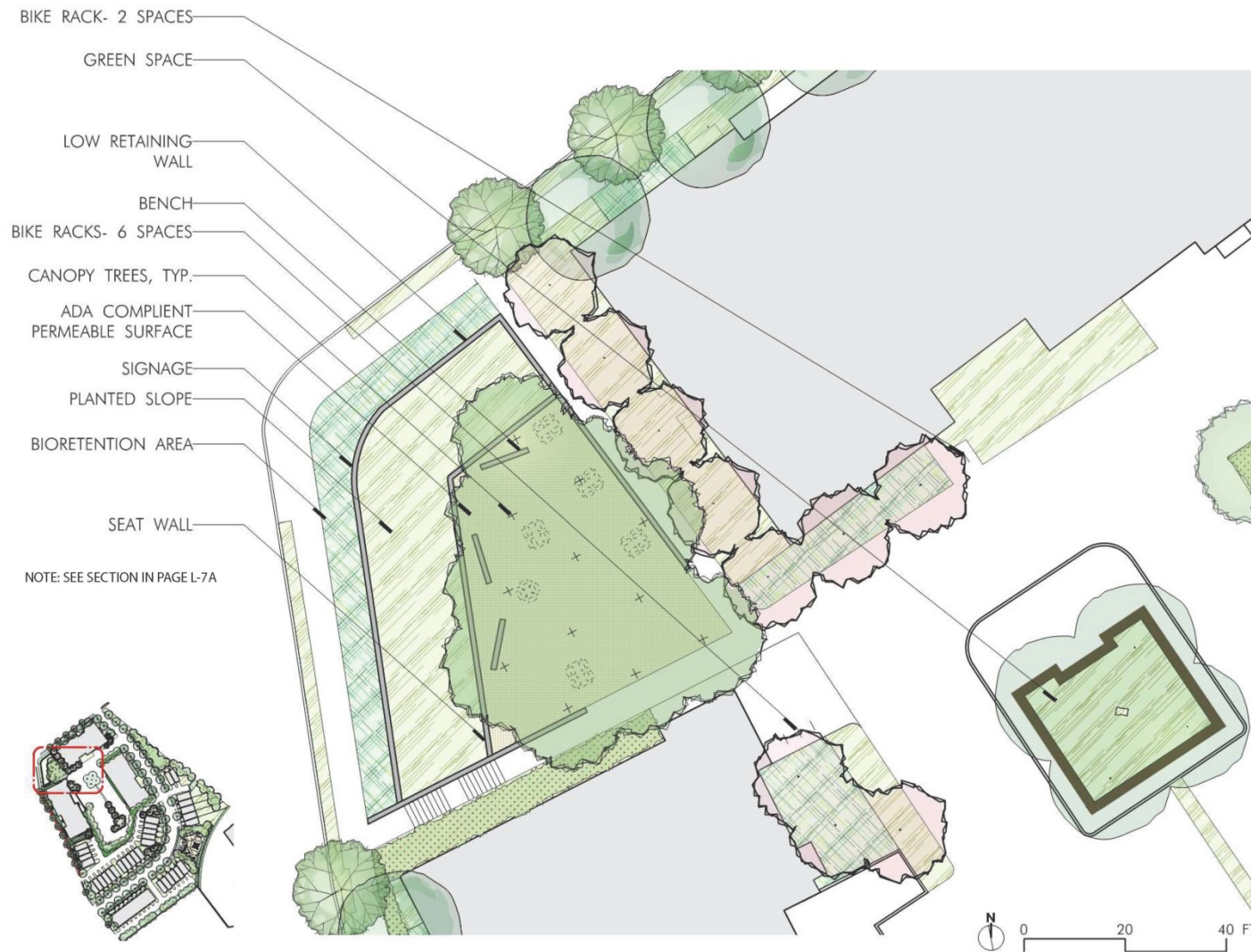
Bioretention areas
