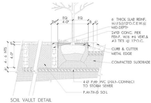
SOIL VAULT DETAIL
