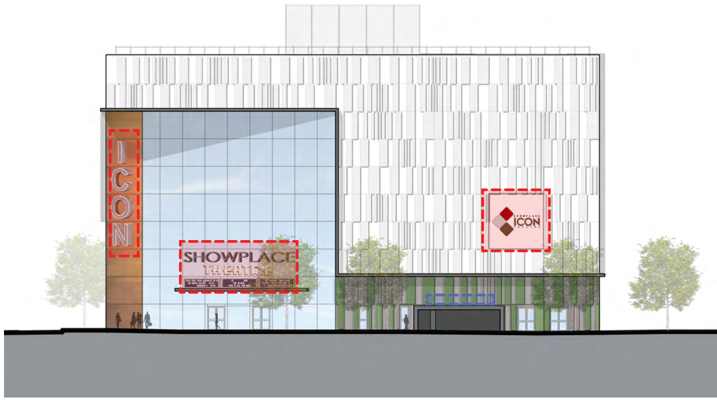
West Elevation - 1 1/2 Street
