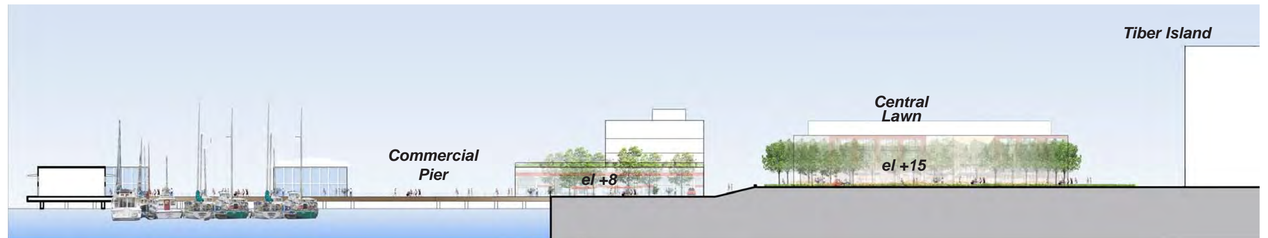
SECTION THROUGH WATERFRONT PARK 0' 32' 64'
