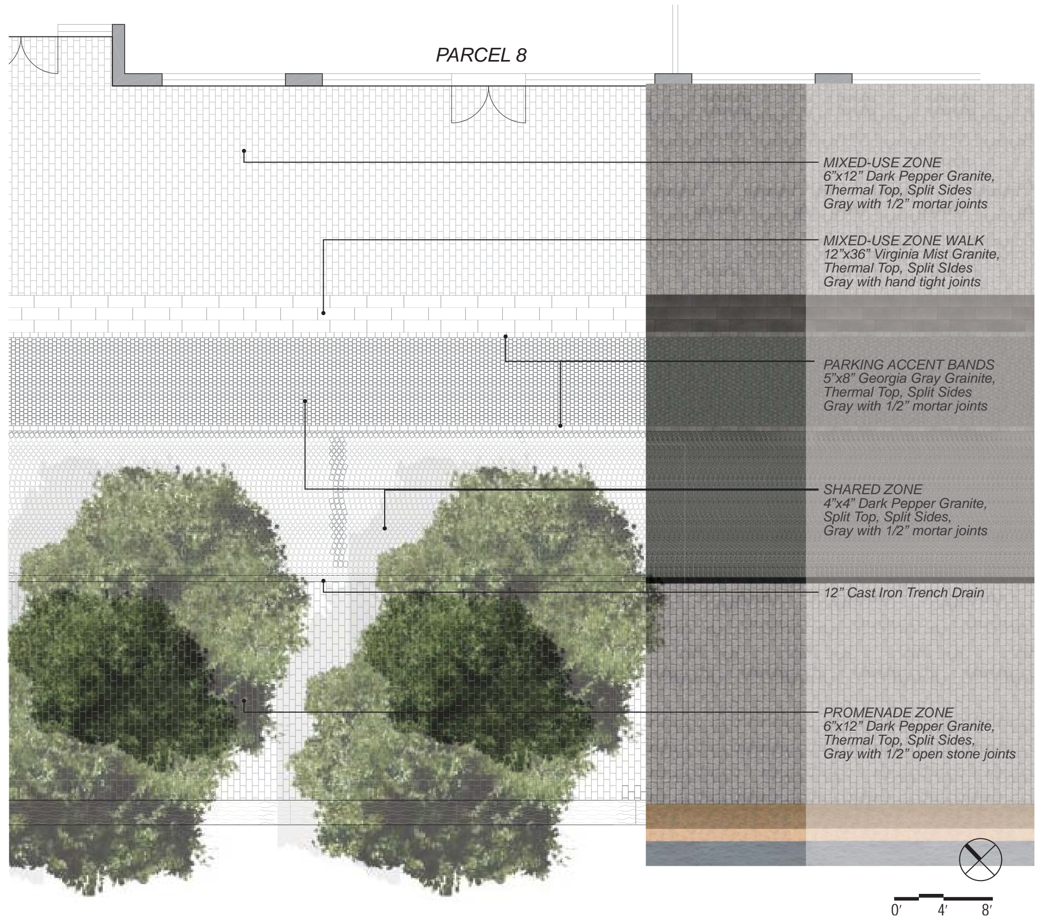
Parking Accent Bands: 5"x8" Georgia Gray Granite Pavers
