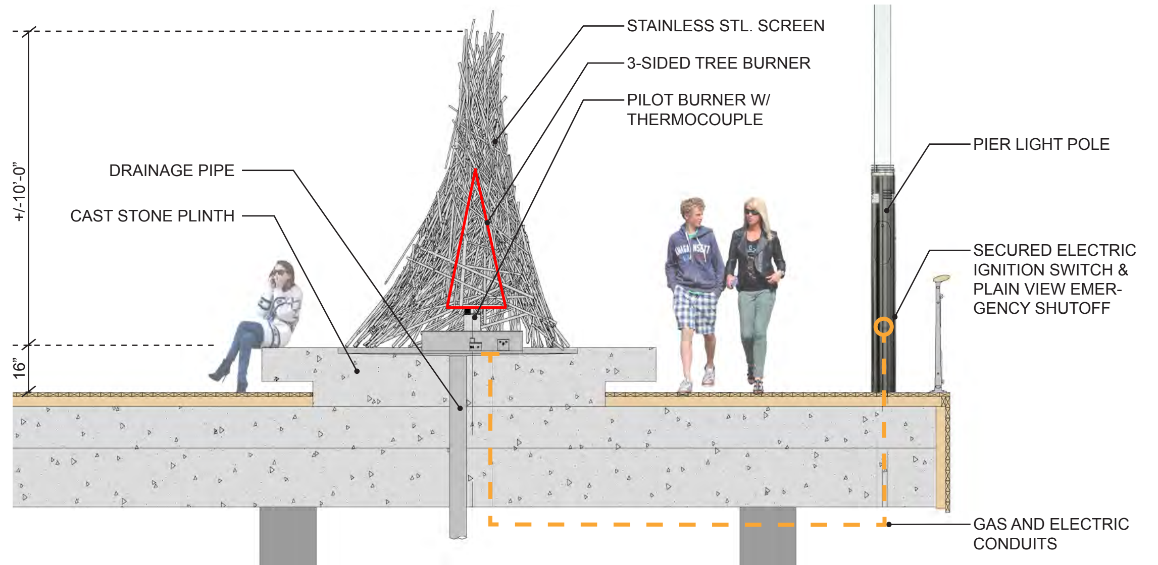
SECTION DETAIL
