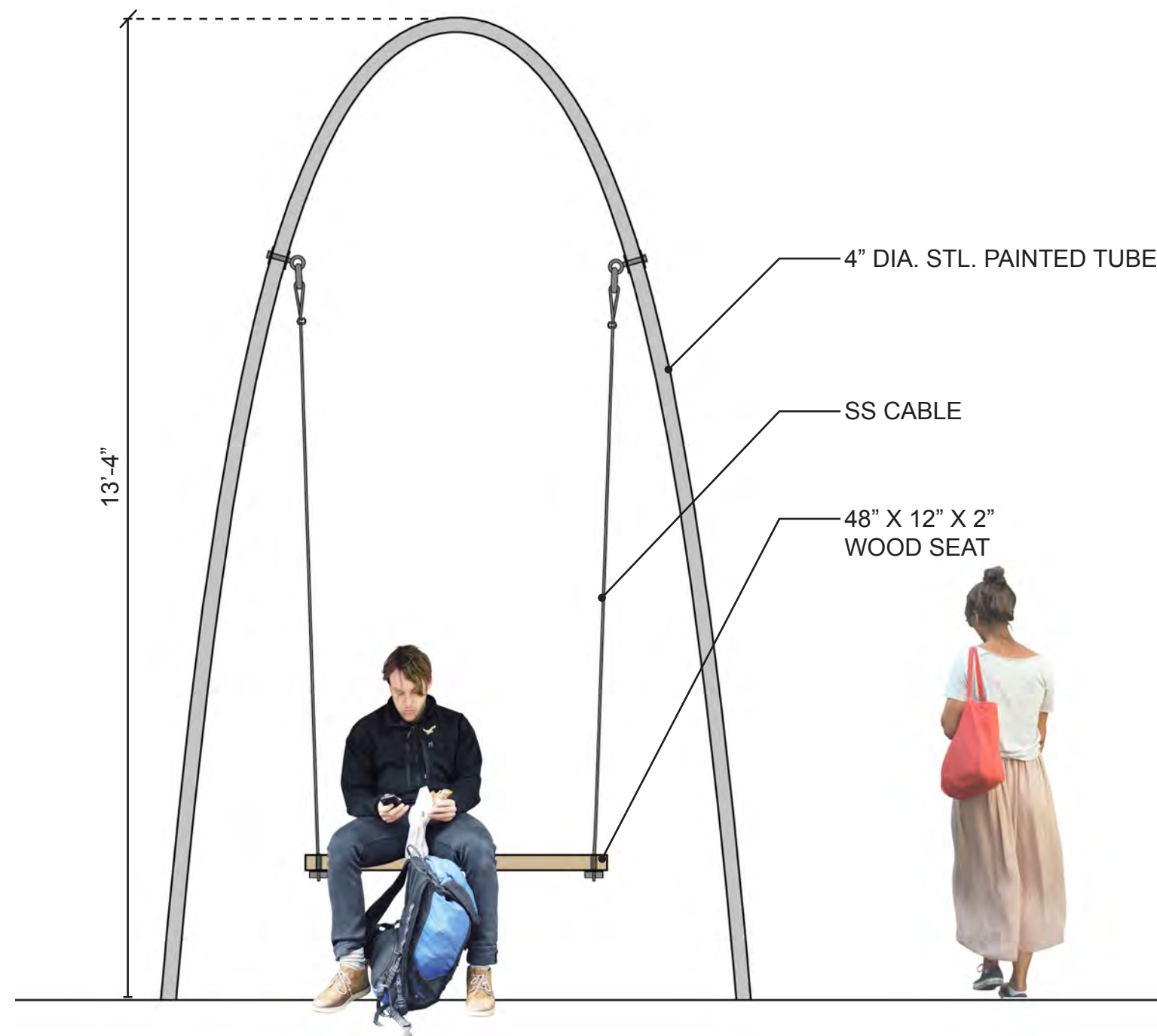
SWING ELEVATION
