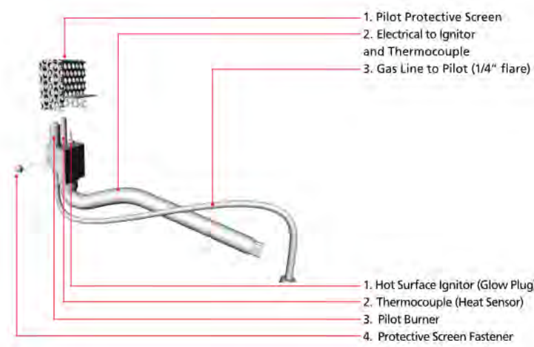
PILOT BURNER ASSEMBLY
