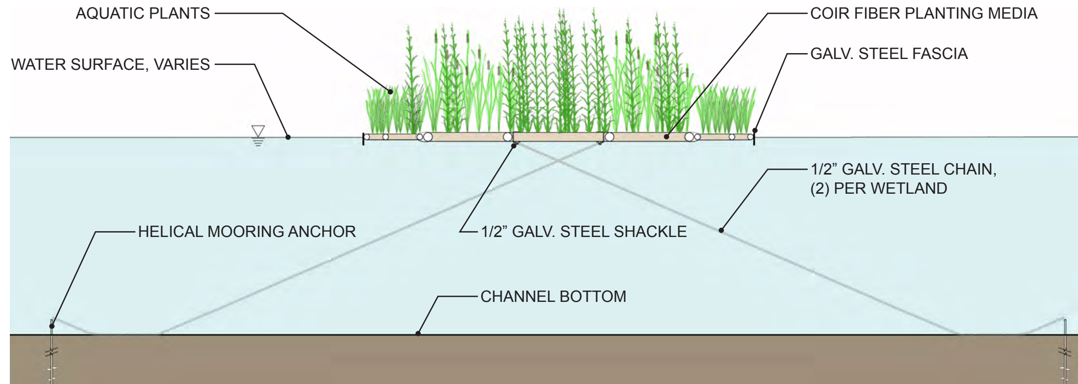
FLOATING WETLAND SECTION
