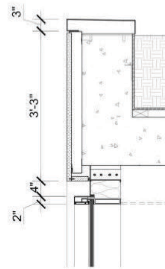
2. DETAIL SECTION
