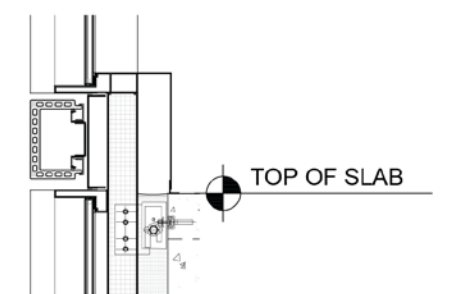
1. DETAIL SECTION
