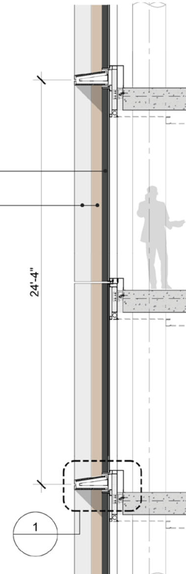
SECTION
