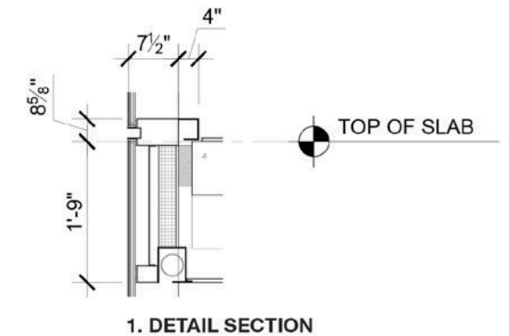
1. DETAIL SECTION
