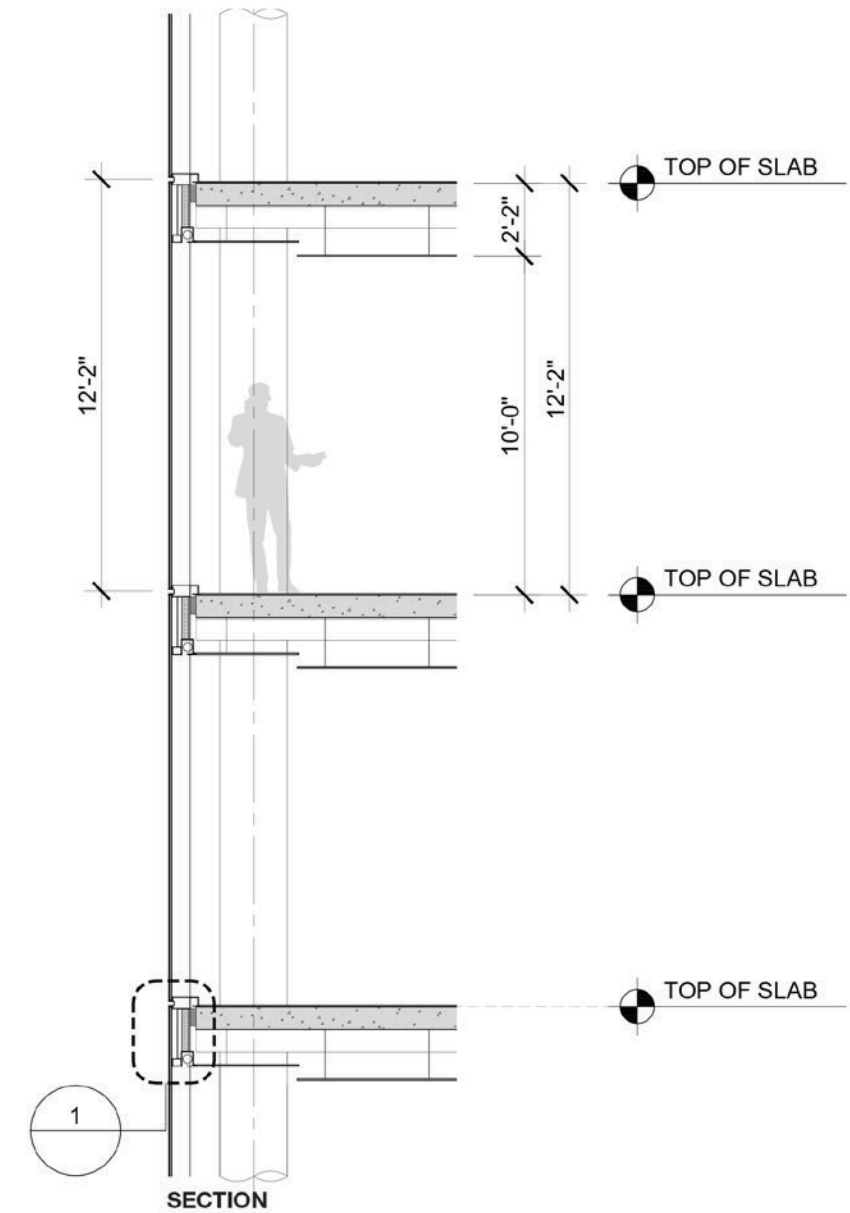
SECTION
