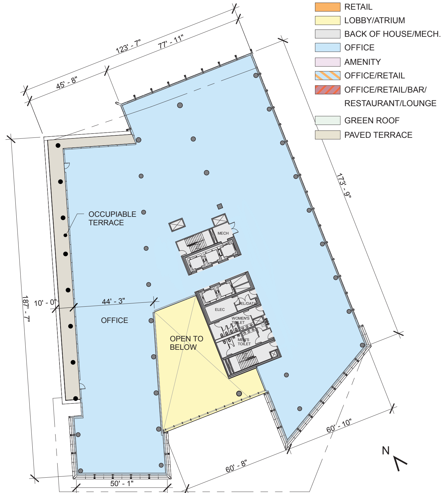
3RD FLOOR
