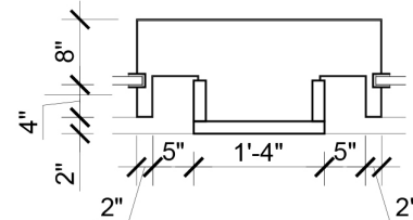
1. DETAIL PLAN
