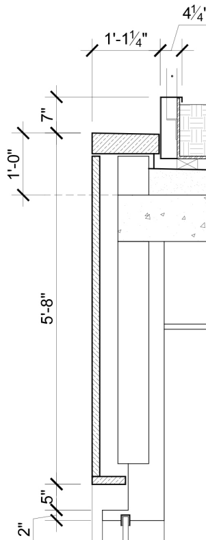
2. DETAIL SECTION
