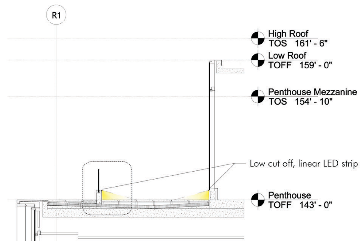
SECTION A
