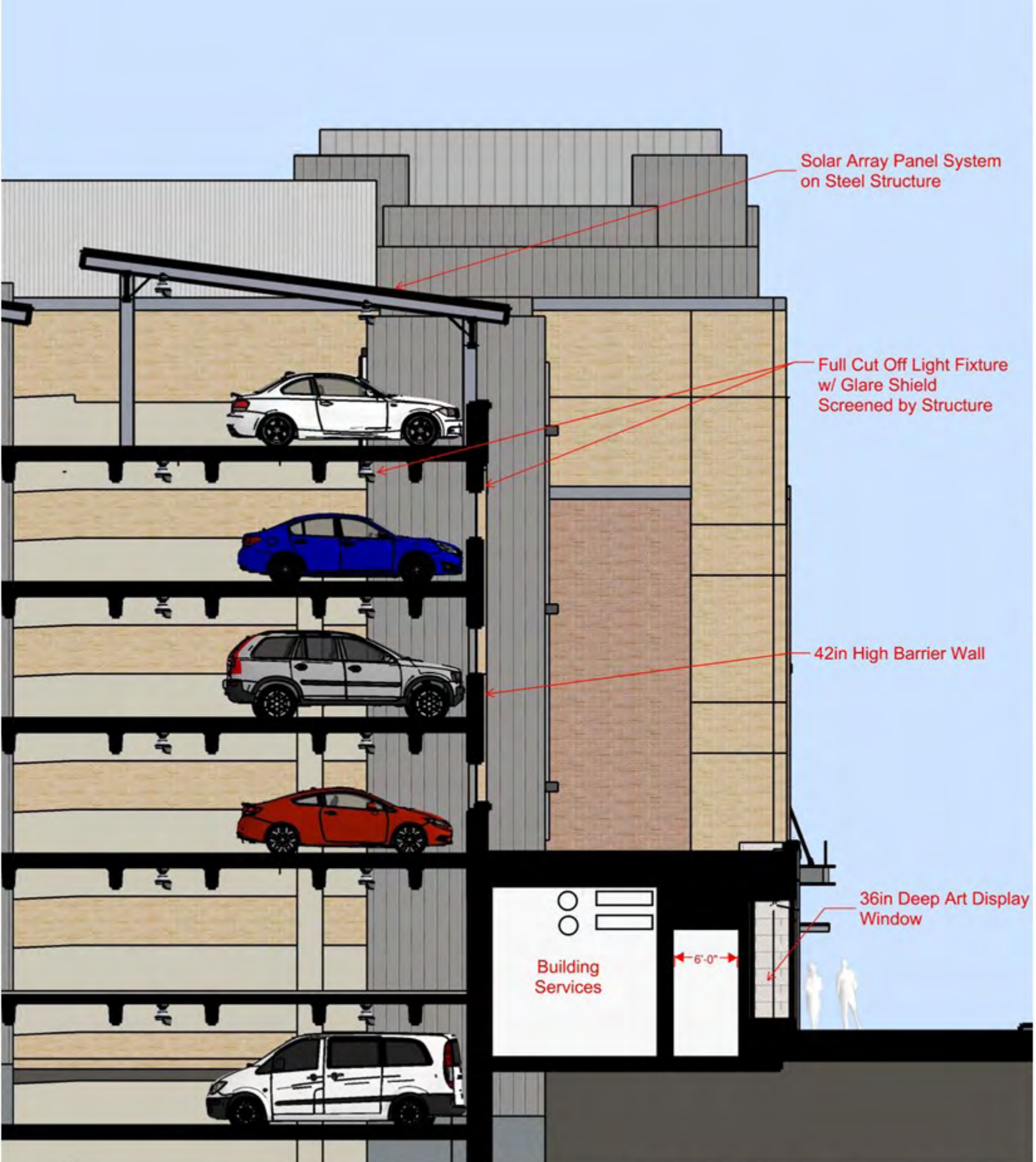
GARAGE SECTION AT NAYLOR ROAD
