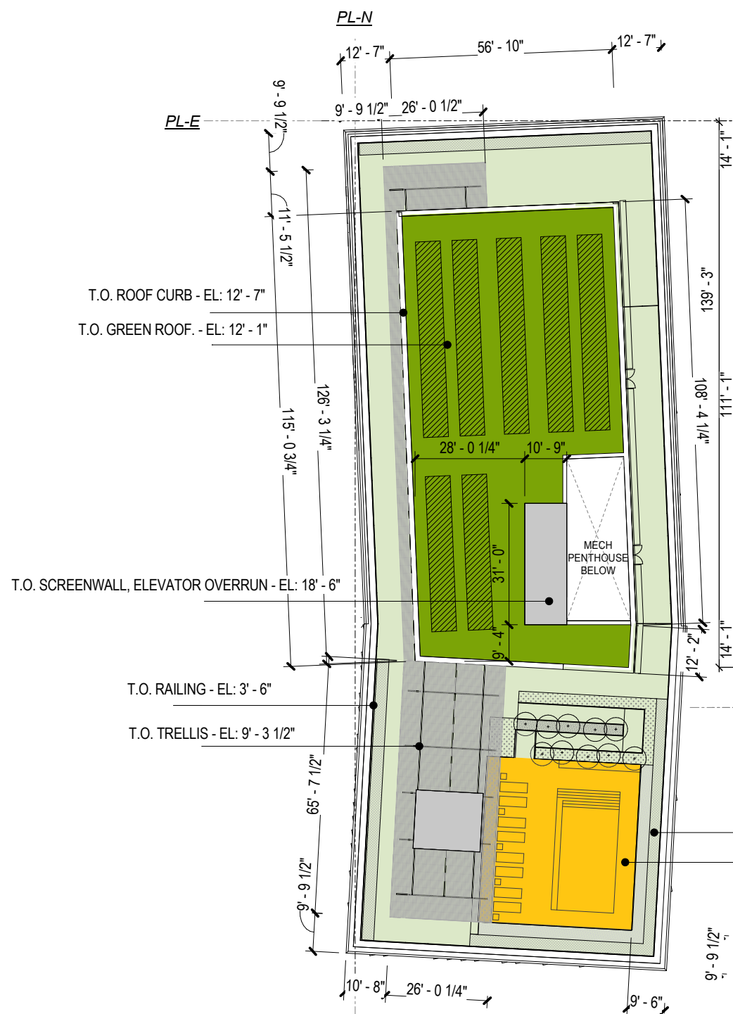
RESIDENTIAL PENTHOUSE PLAN
