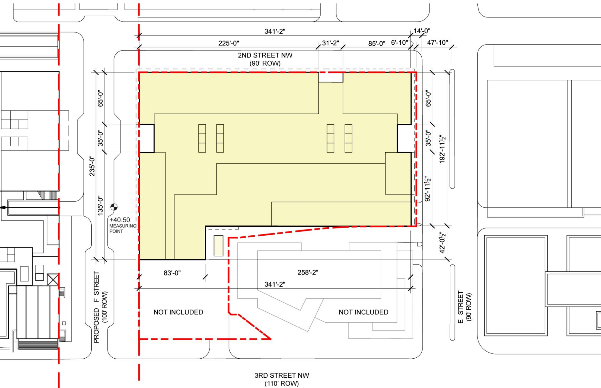
South Block - Site Plan
