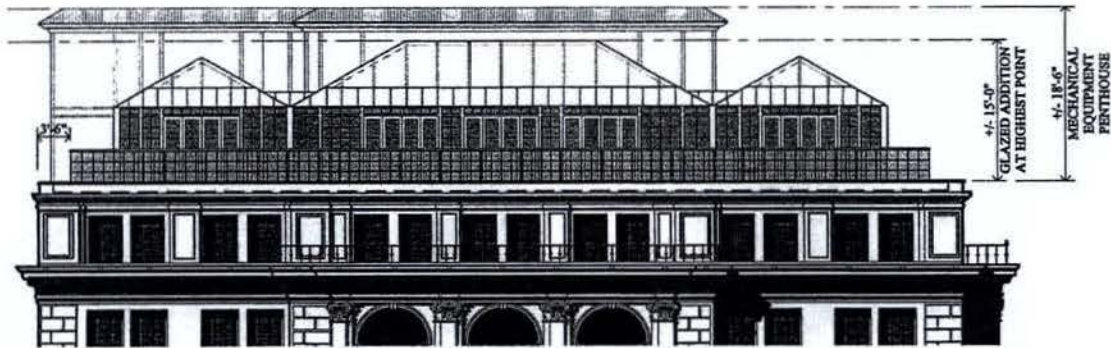
SOUTH ELEVATION WITH GUARD RAIL (SET BACK 3'-6")
