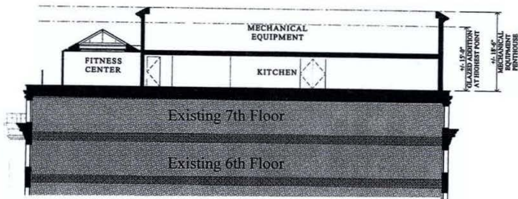
East West Section looking South
