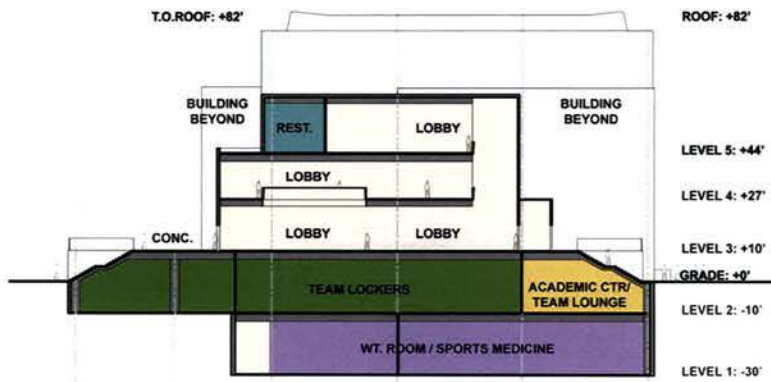
TRANSVERSE SECTION LOOKING NORTH
