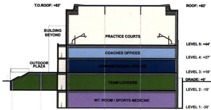
TRANSVERSE SECTION LOOKING NORTH
