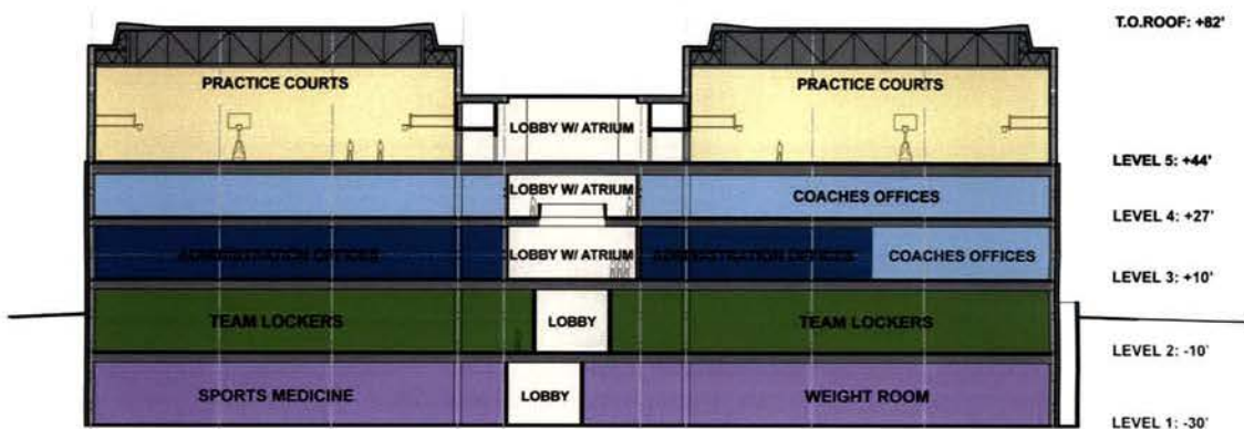
LONGITUDINAL SECTION LOOKING WEST
