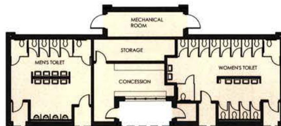
Visitor Side Concessions / Toilets Building Floor Plan
