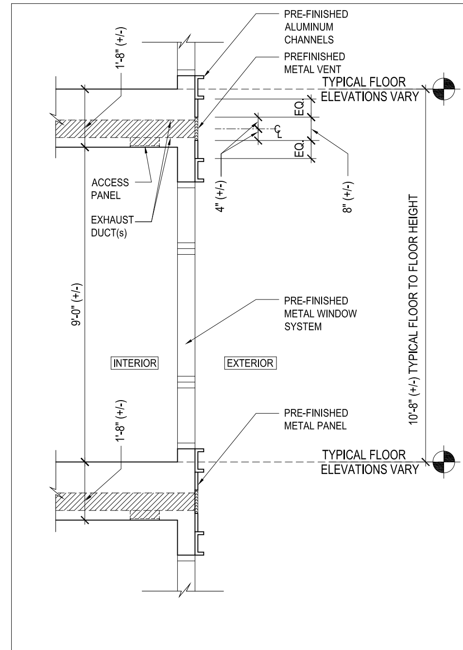
1 SECTION DETAIL AT METAL VENT
