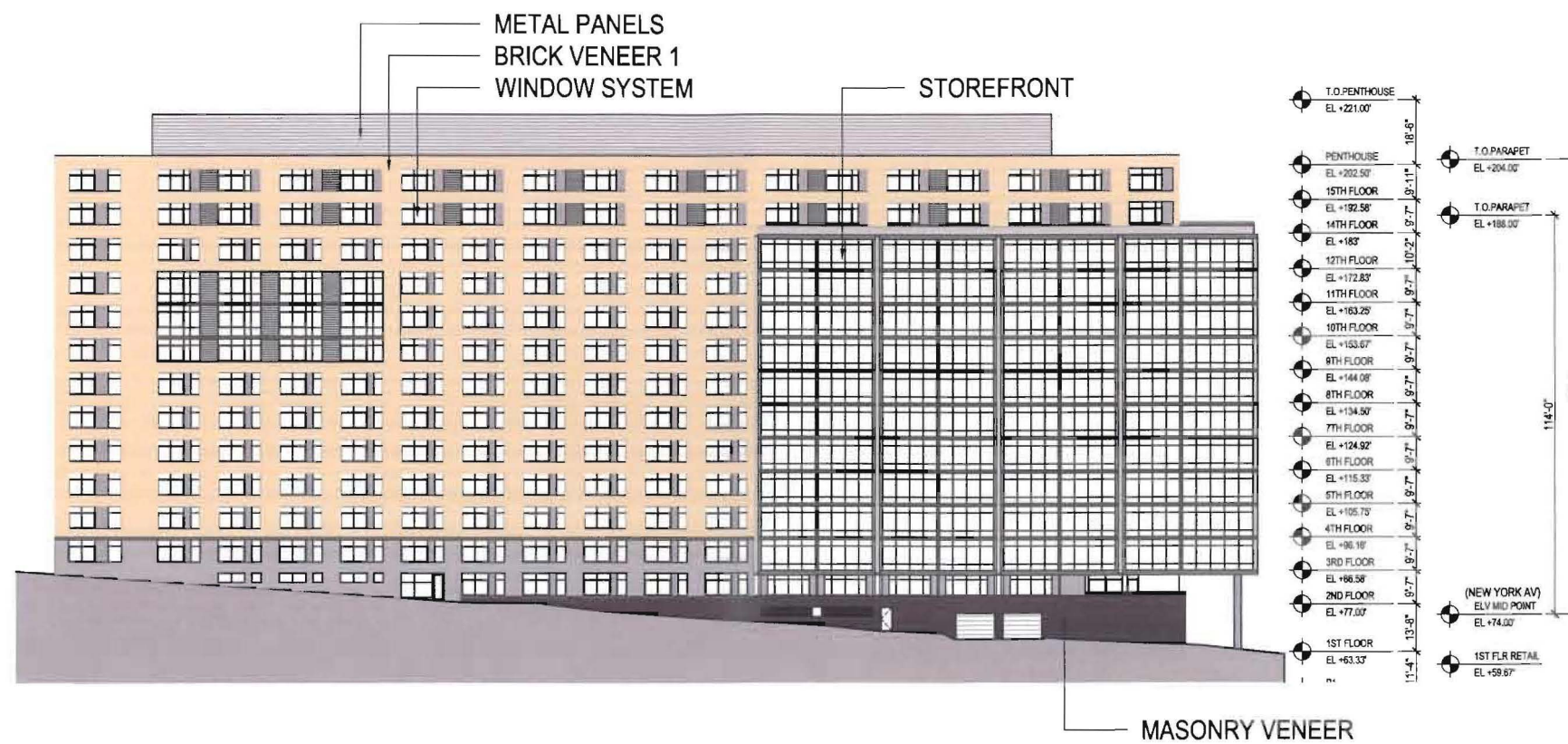
1 North Elevation
