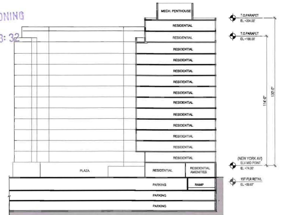
2 Section B-B
