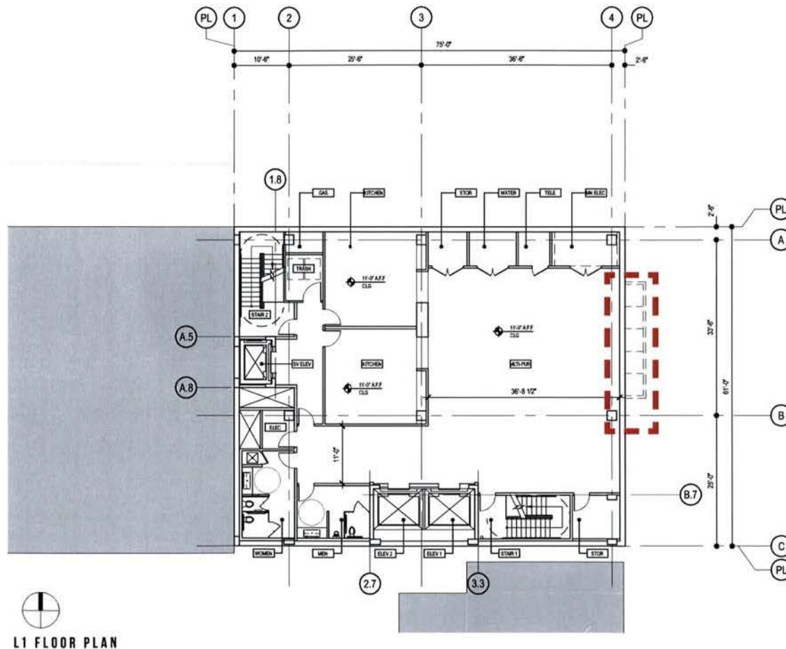
AREAWAY, STRUCTURAL GLASS ROOF
