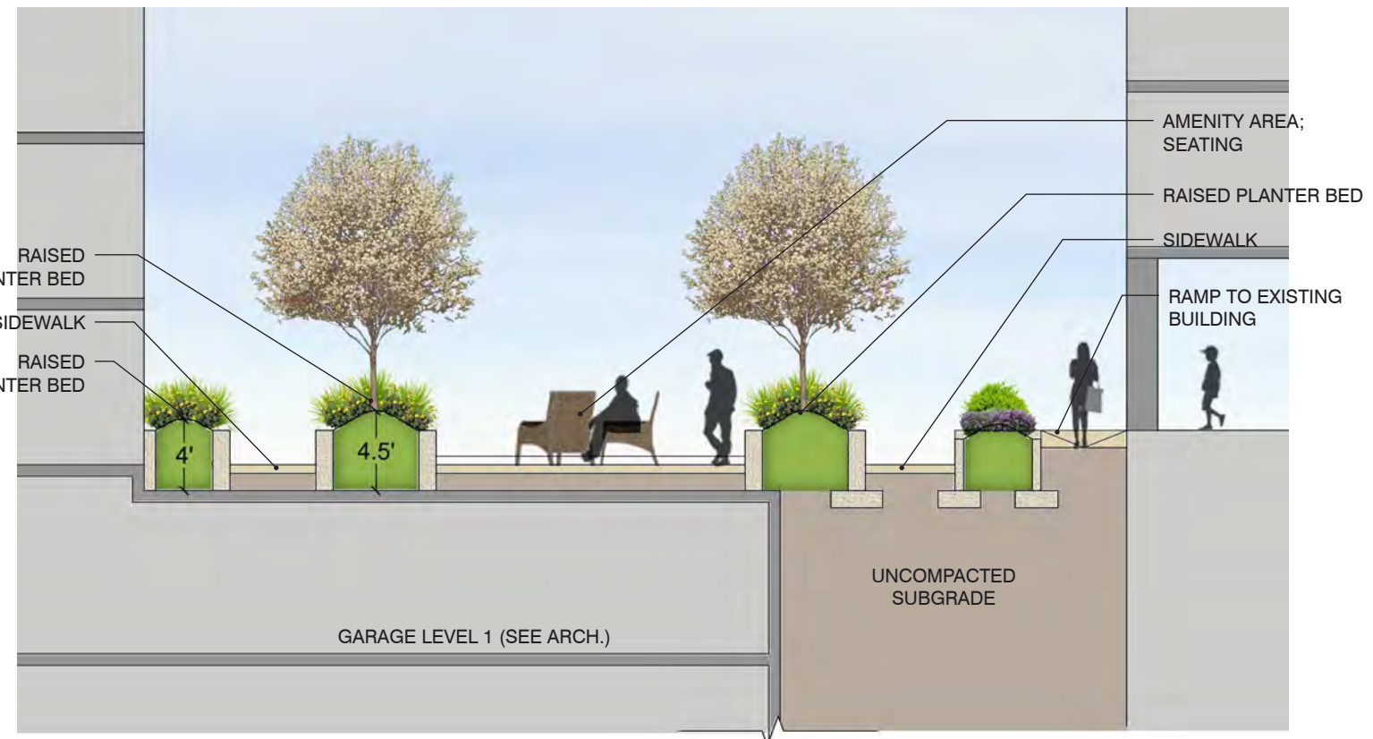
2 SECTION - SOUTH COURTYARD B-B'
