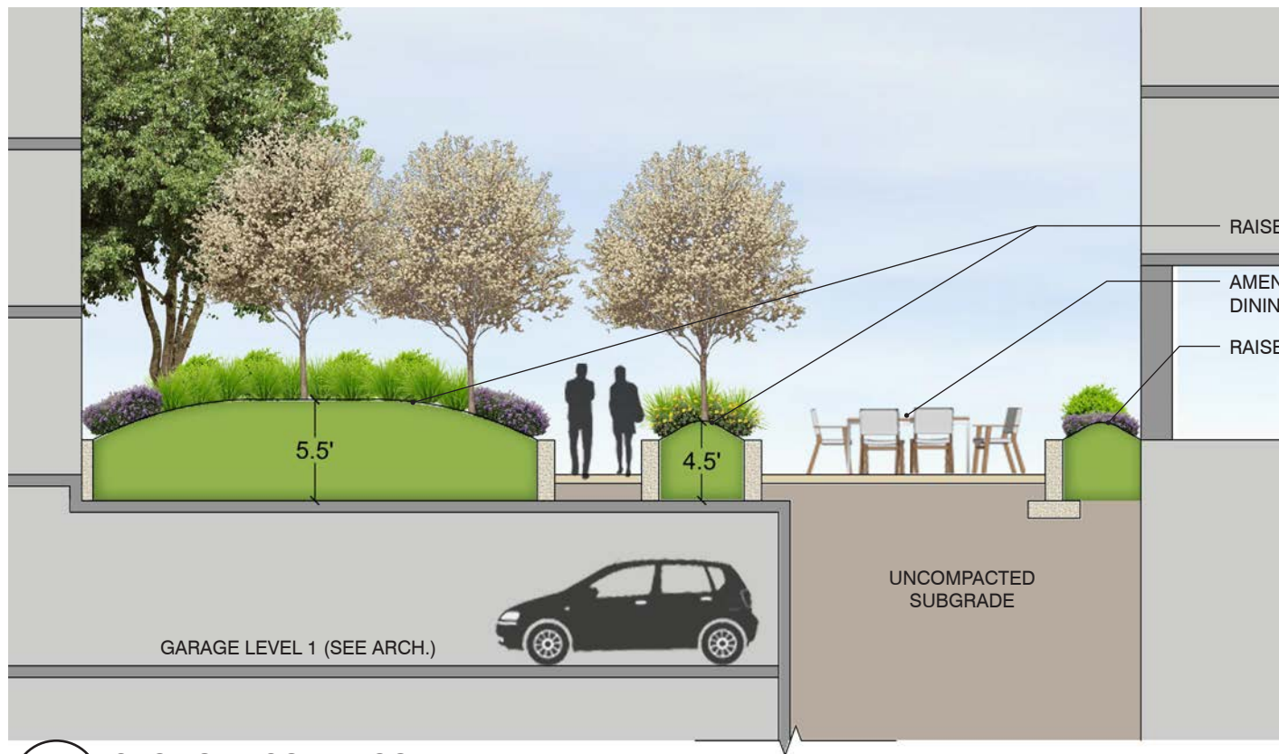
1 SECTION - SOUTH COURTYARD A-A' L-17
