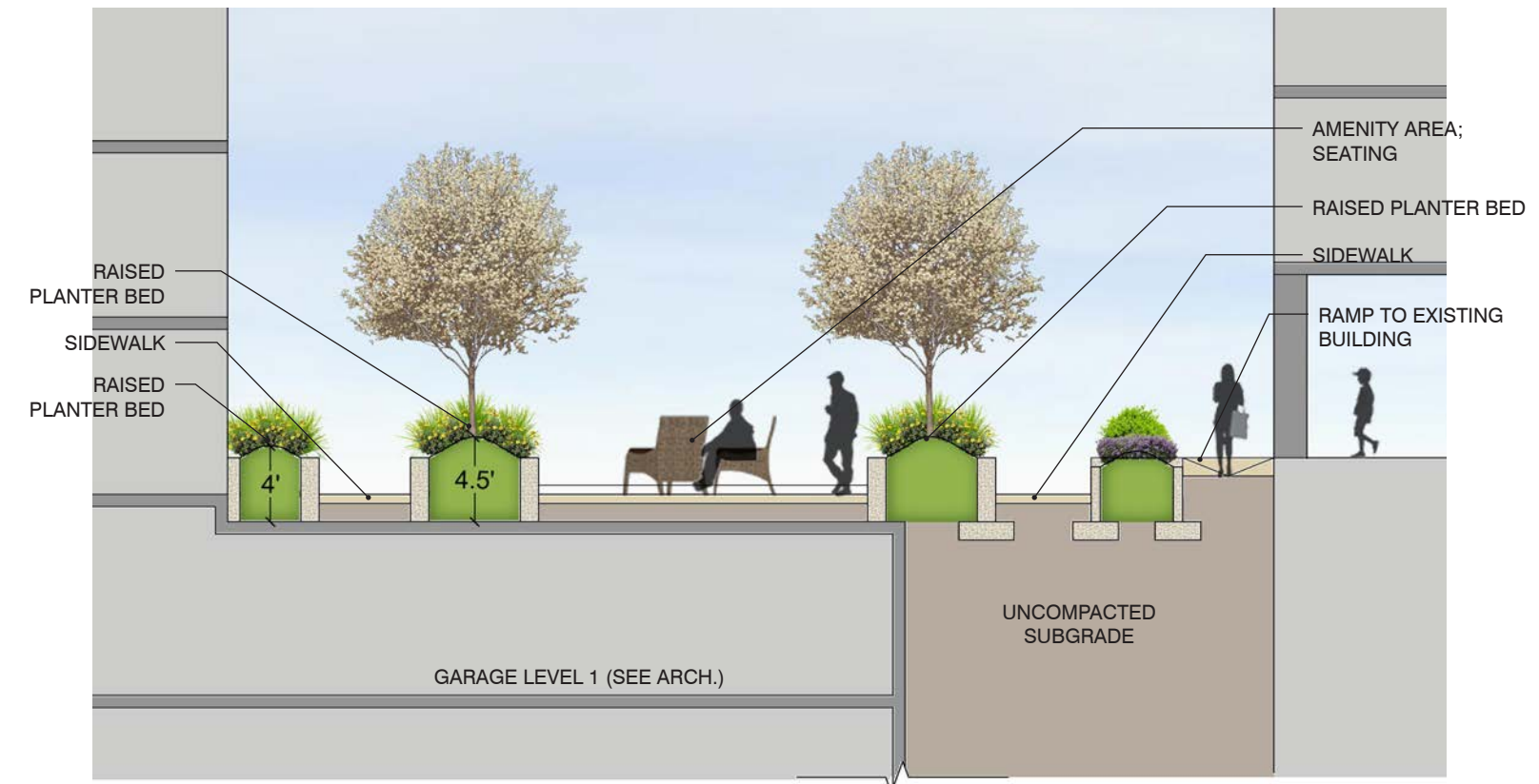
3 SECTION - SOUTH COURTYARD C-C' L-17
