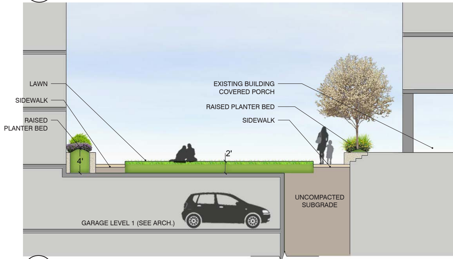
2 SECTION - SOUTH COURTYARD B-B' L-17
