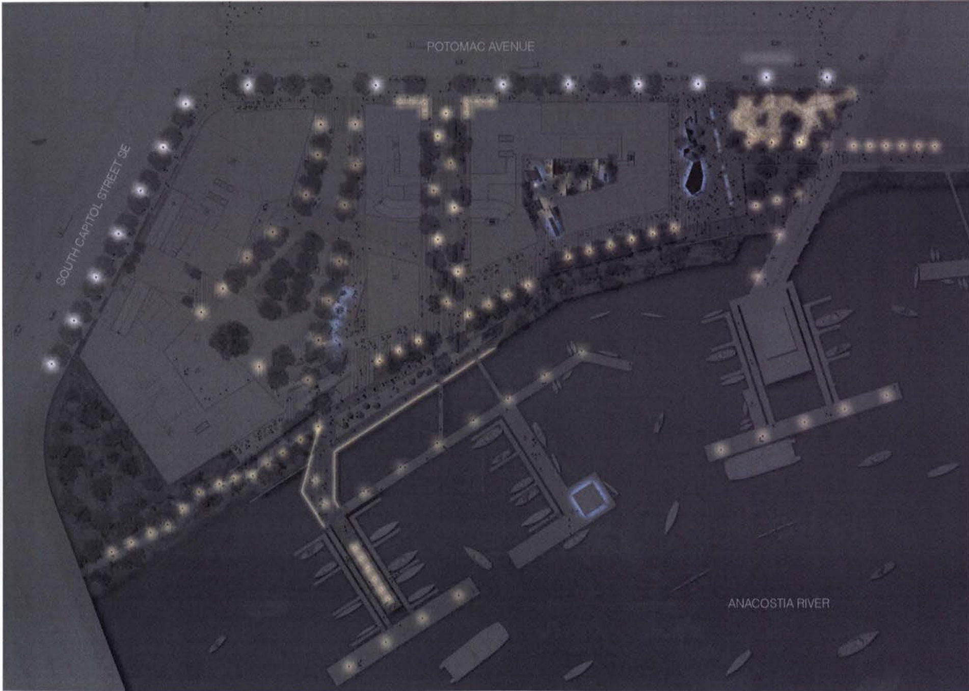
Site Lighting Plan
