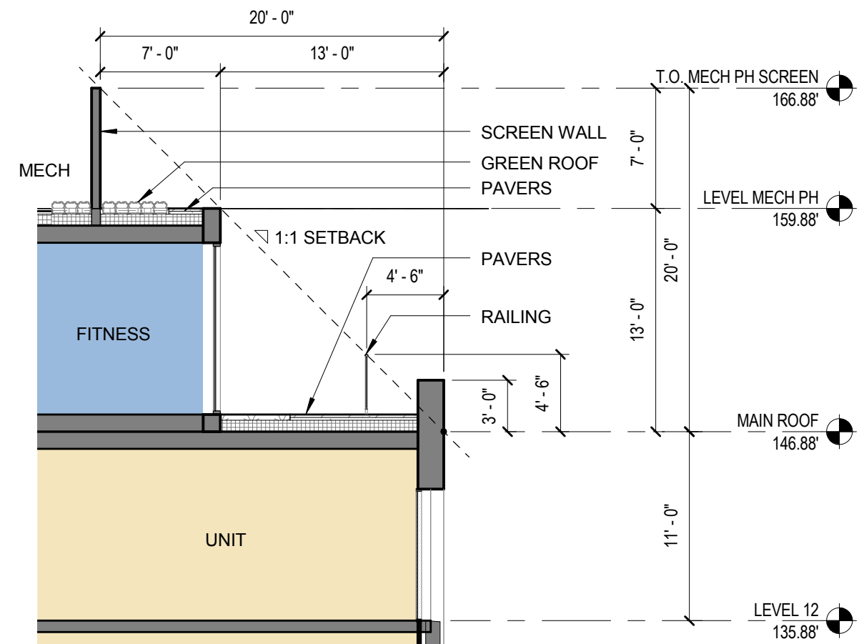
2 ENLARGED SECTION 2 1/8" = 1'-0"
