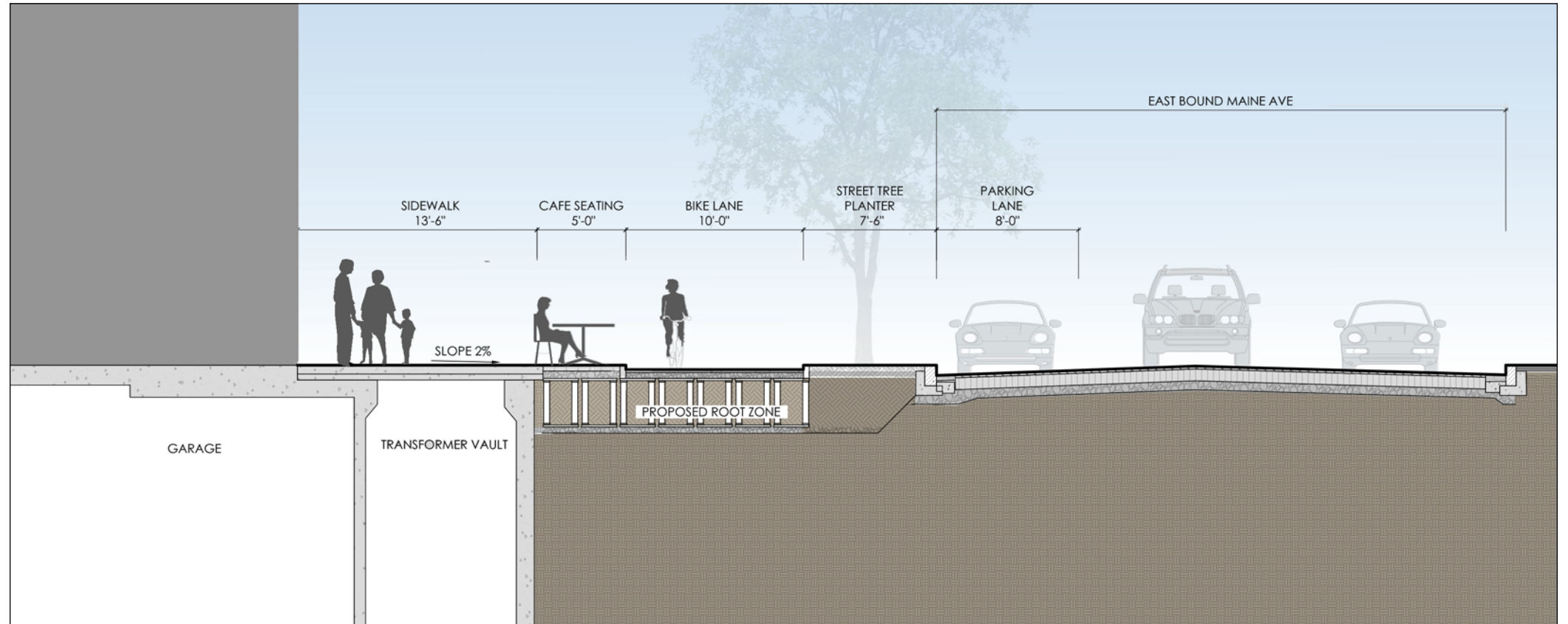
Section at Parcel 7 Flexible Cafe Zone
