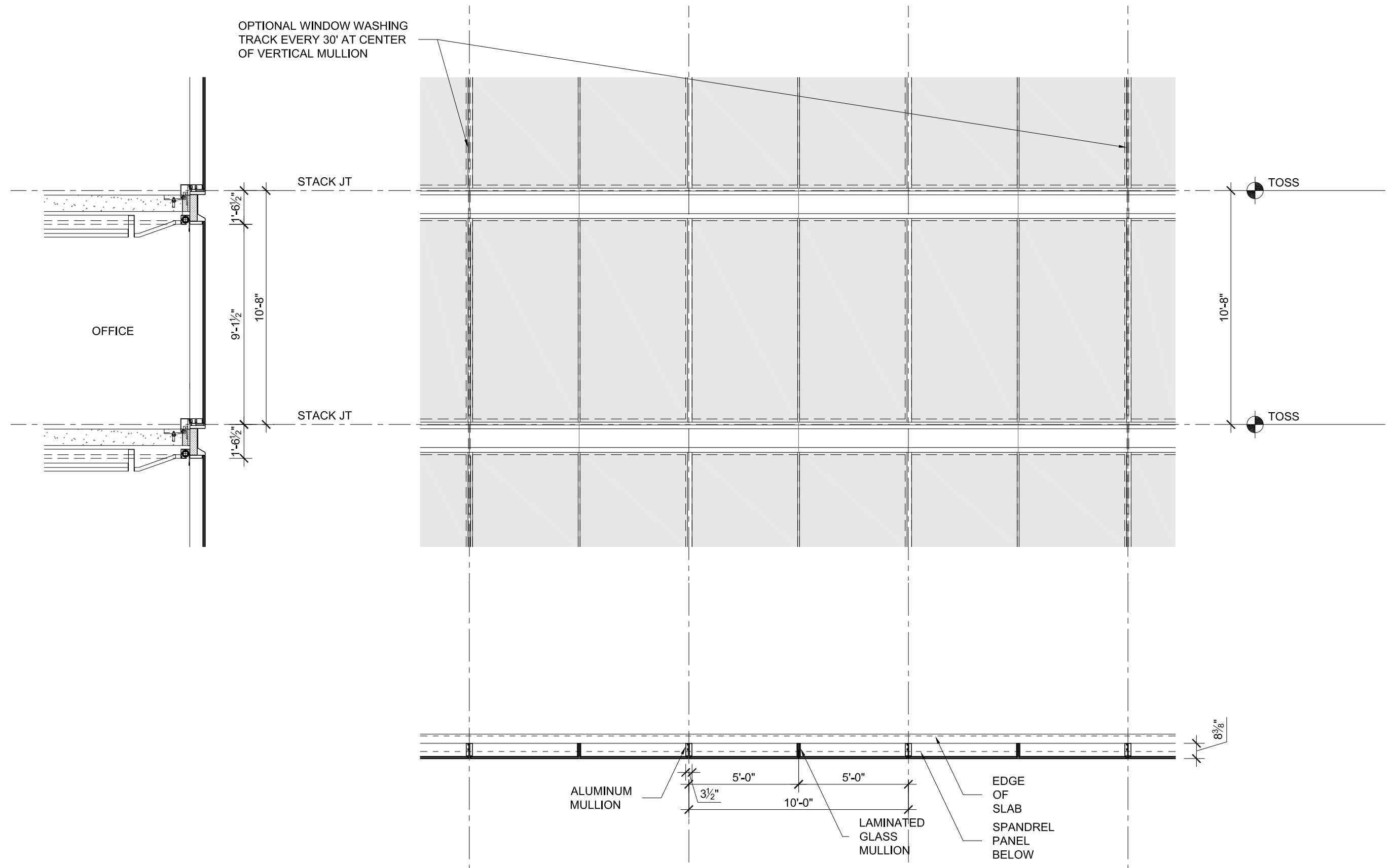
Exterior Wall Type 1A (Flat Wall, No Glass Fins)
