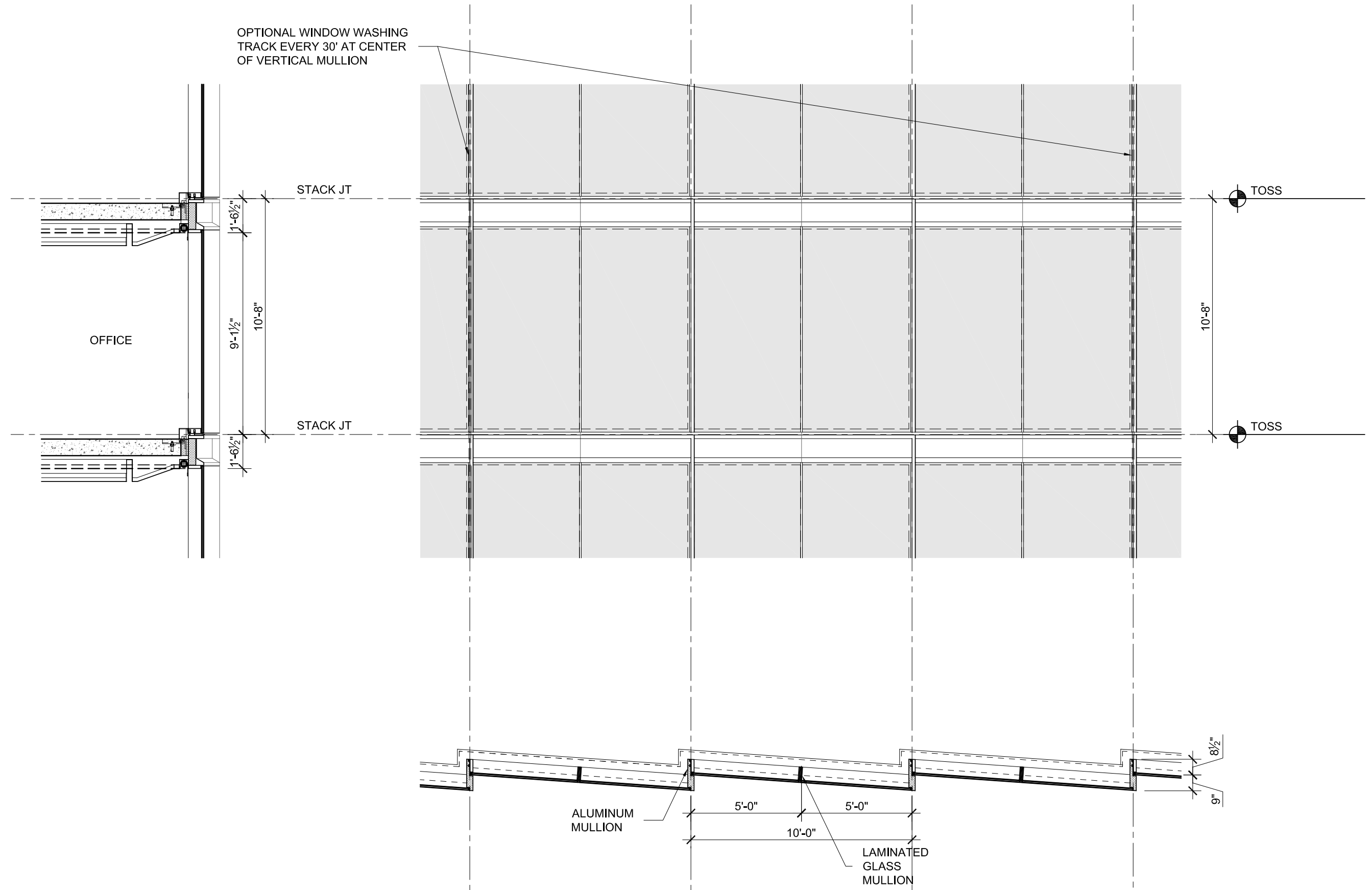
Exterior Wall Type 1B (Angled Wall, No Glass Fins)
