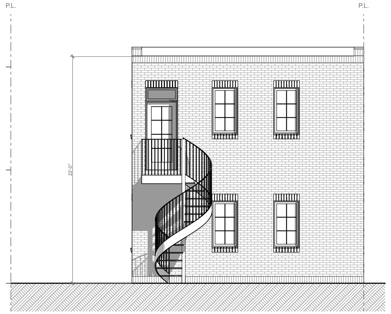
FRONT ELEVATION
