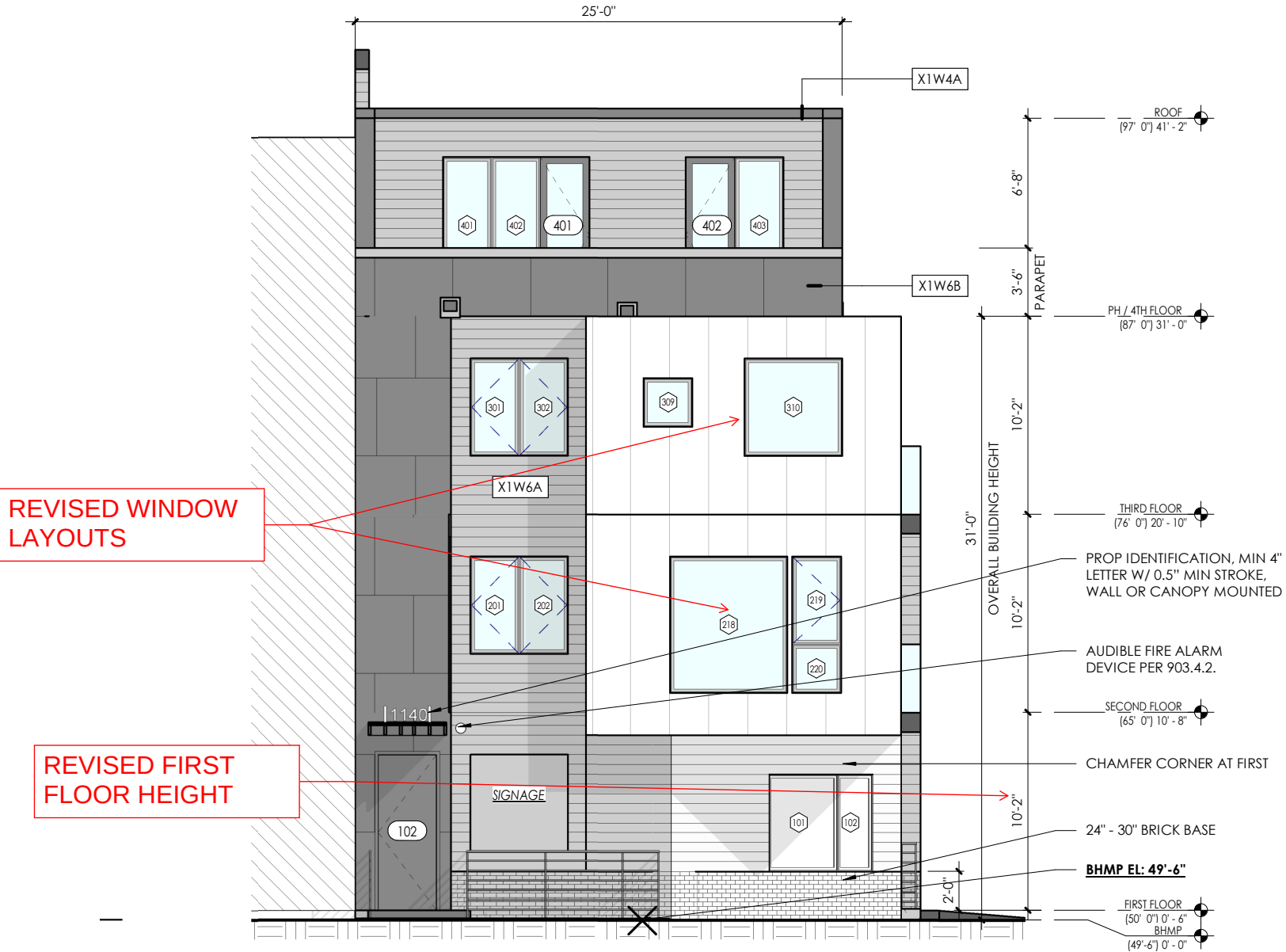
1 NORTHWEST (STREET) ELEVATION 3/16" = 1'-0"
