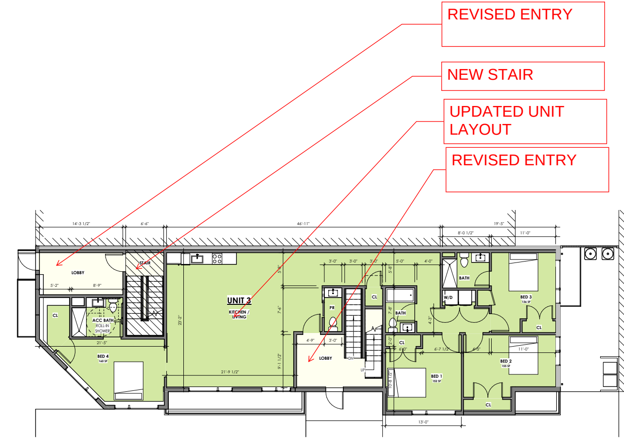
2 FIRST FLOOR 1/8" = 1'-0"
