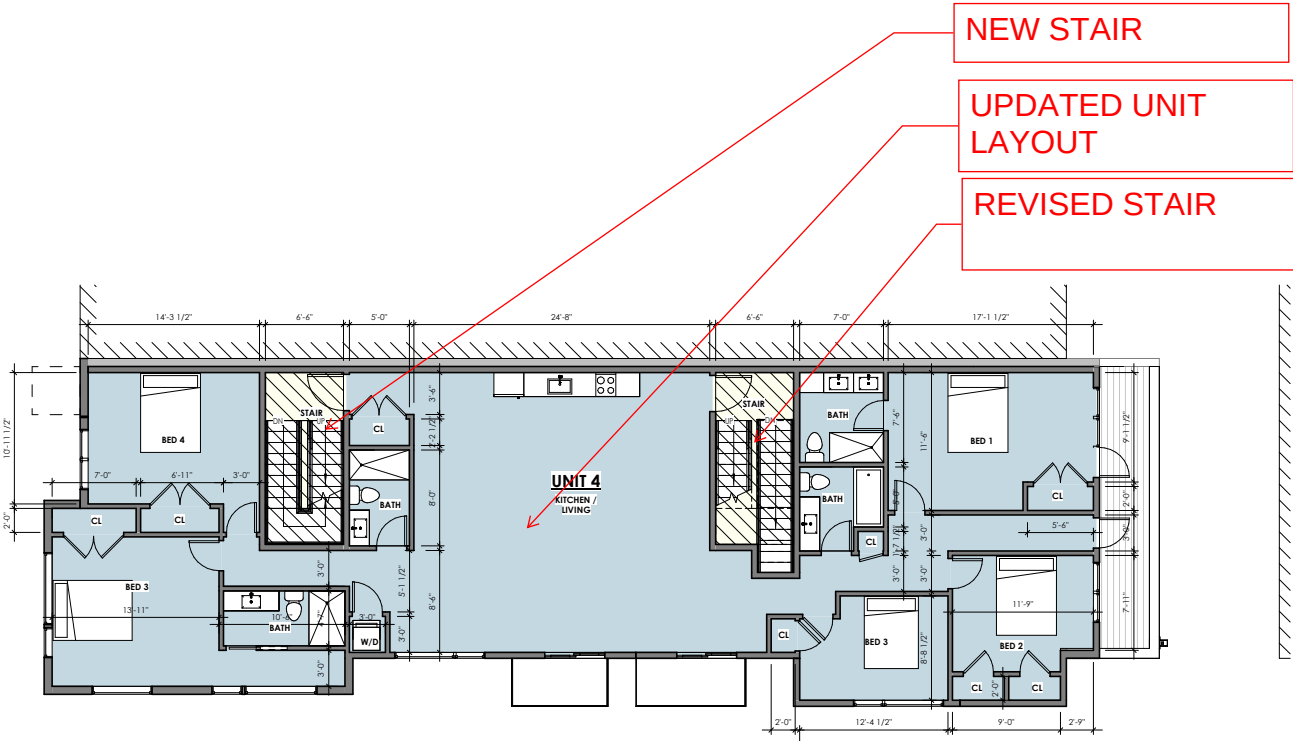
3 SECOND FLOOR 1/8" = 1'-0"
