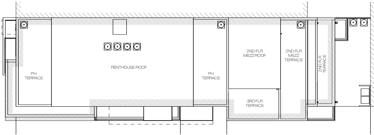
6 ROOF PLAN
