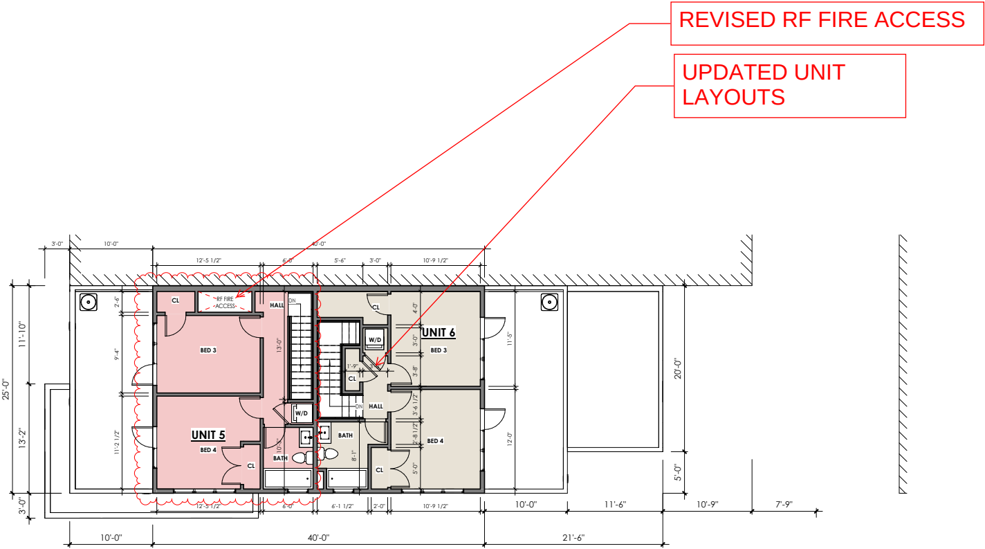
5 PENTHOUSE / 4TH FLOOR 1/8" = 1'-0"
