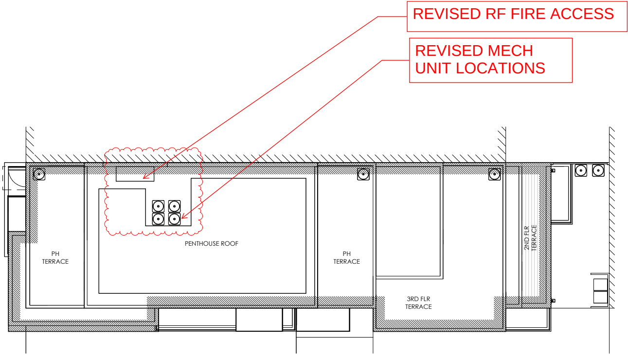
6 ROOF PLAN 1/8" = 1'-0"
