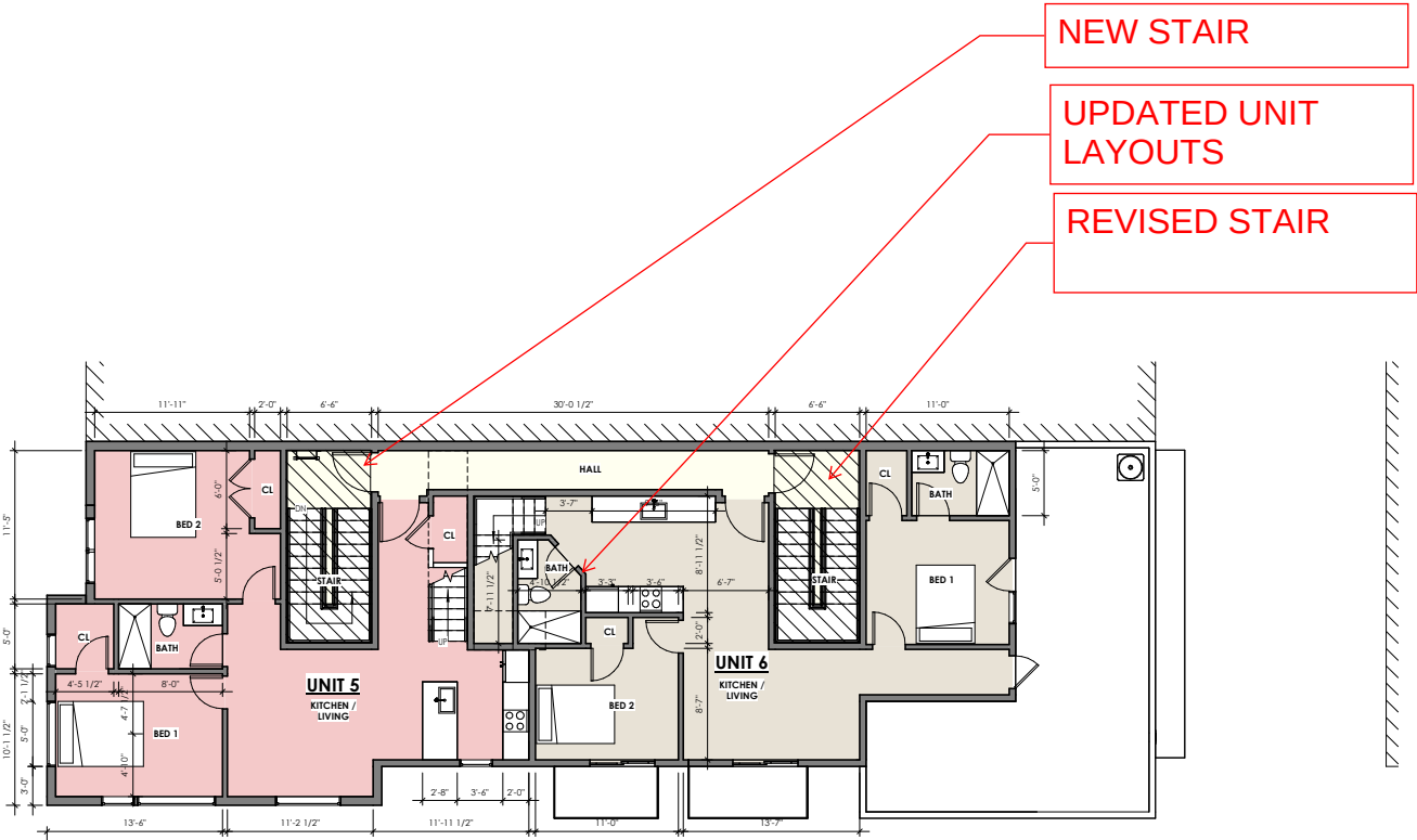
4 THIRD FLOOR 1/8" = 1'-0"
