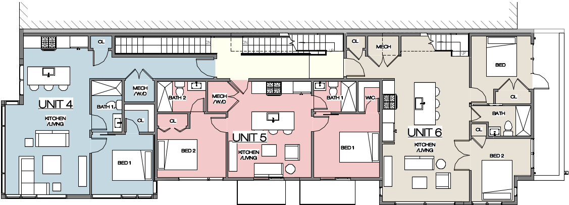
3 SECOND FLOOR
