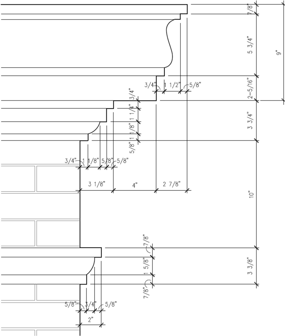
Cornice Detail
