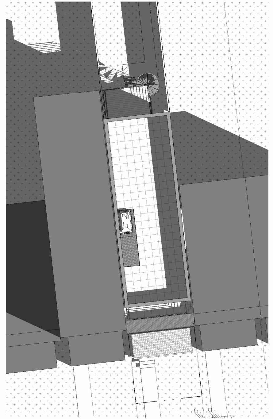
1 SOLAR STUDY PLAN - SEP. 21 - 930 AM C202 | B503 1/16" = 1'-0"
