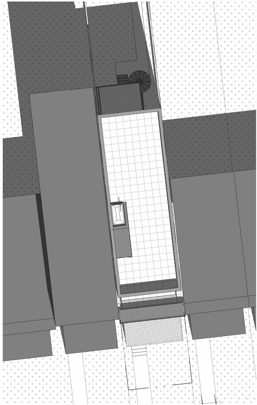
2 SOLAR STUDY PLAN - SEP. 21 - 1230 PM C202 | B503 1/16" = 1'-0"
