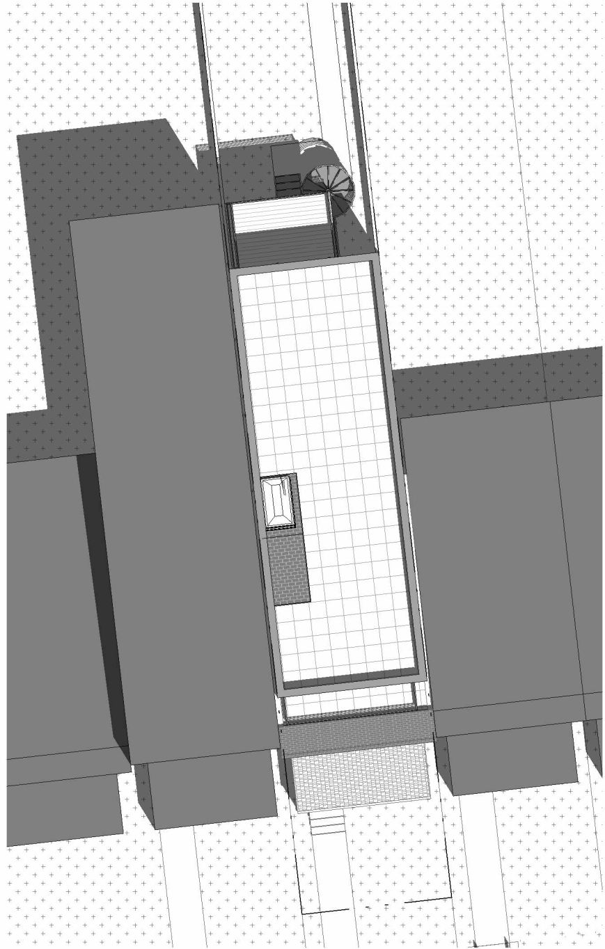
3 SOLAR STUDY PLAN - JUNE 21 - 1230 PM C202 | B502 1/16" = 1'-0"
