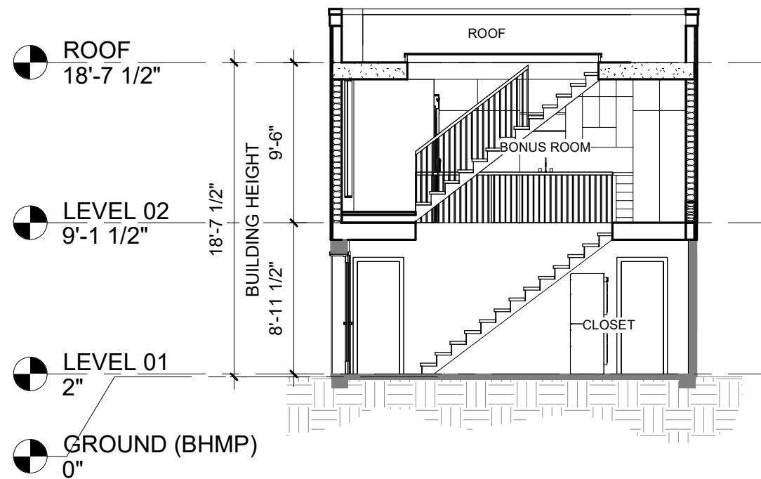
1 NORTH - SOUTH 1/8" = 1'-0"
