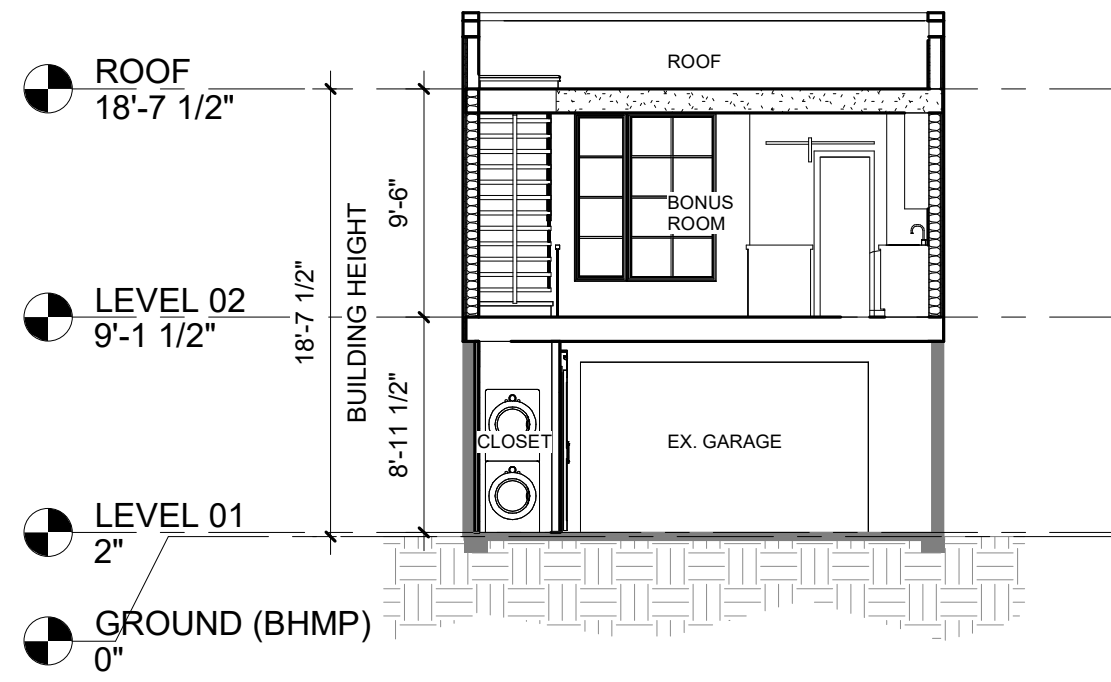
2 WEST - EAST 1/8" = 1'-0"
