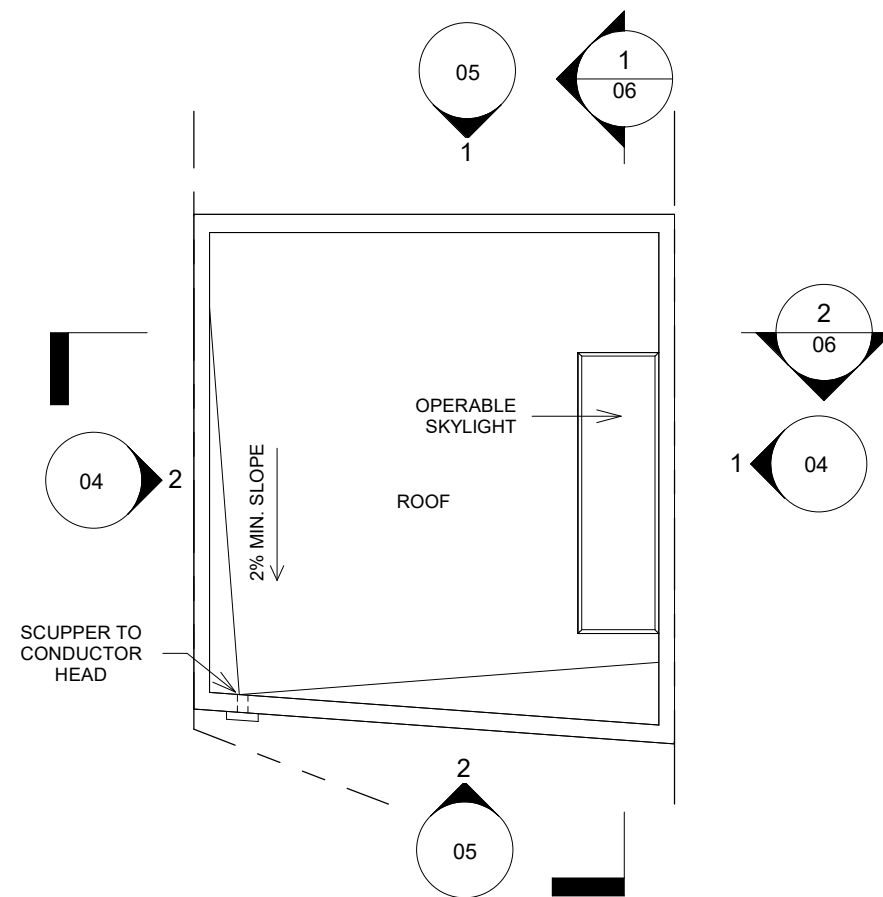
3 ROOF LEVEL 1/8" = 1'-0"
