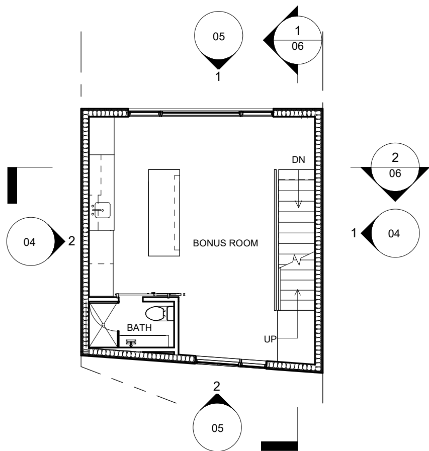
2 LEVEL 2 1/8" = 1'-0"
