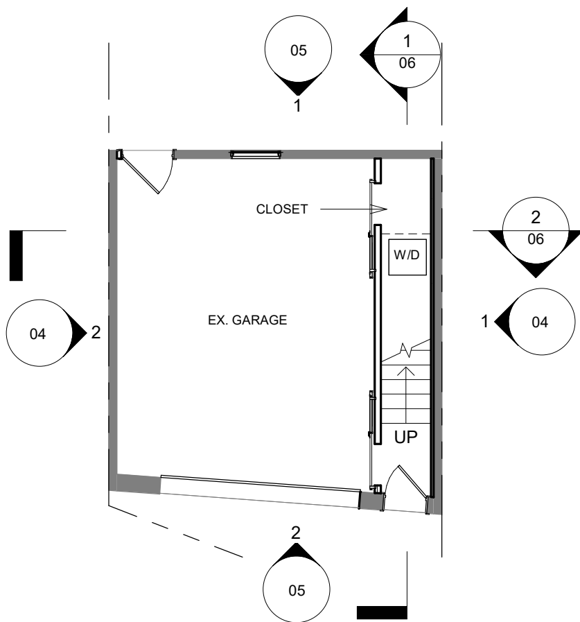
1 LEVEL 1 1/8" = 1'-0"
