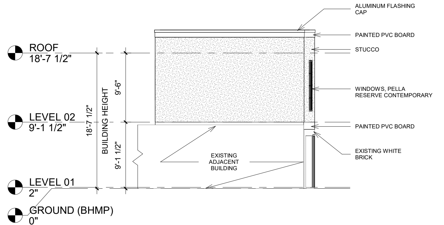
2 ELEVATION - WEST 1/8" = 1'-0"
