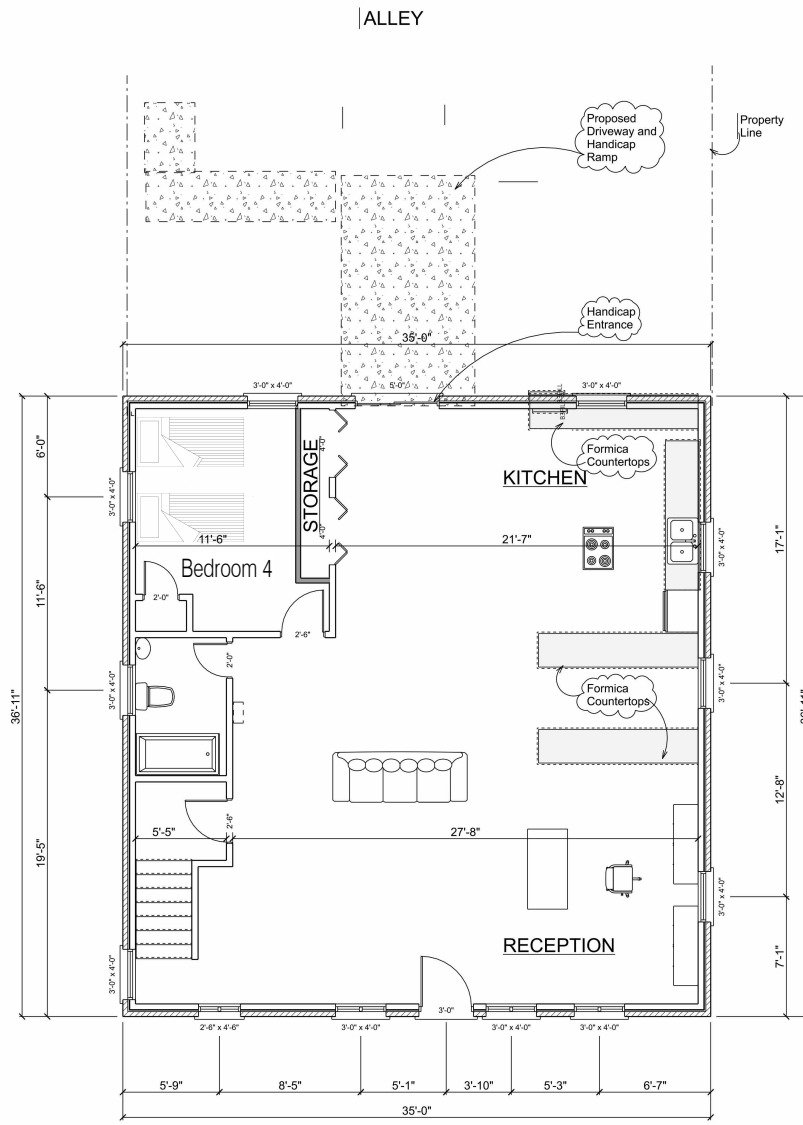
EXISTING/PROPOSED FIRST FLOOR PLAN
